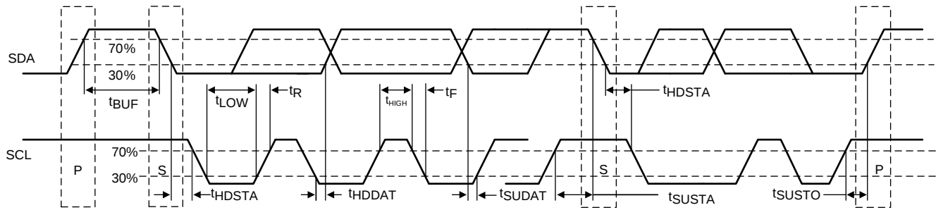
图 1. I²C Timing Diagram Definitions
