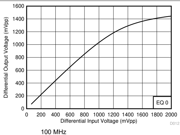
图 5-18. Upstream-to-Downstream Linearity Performance at 100 MHz
