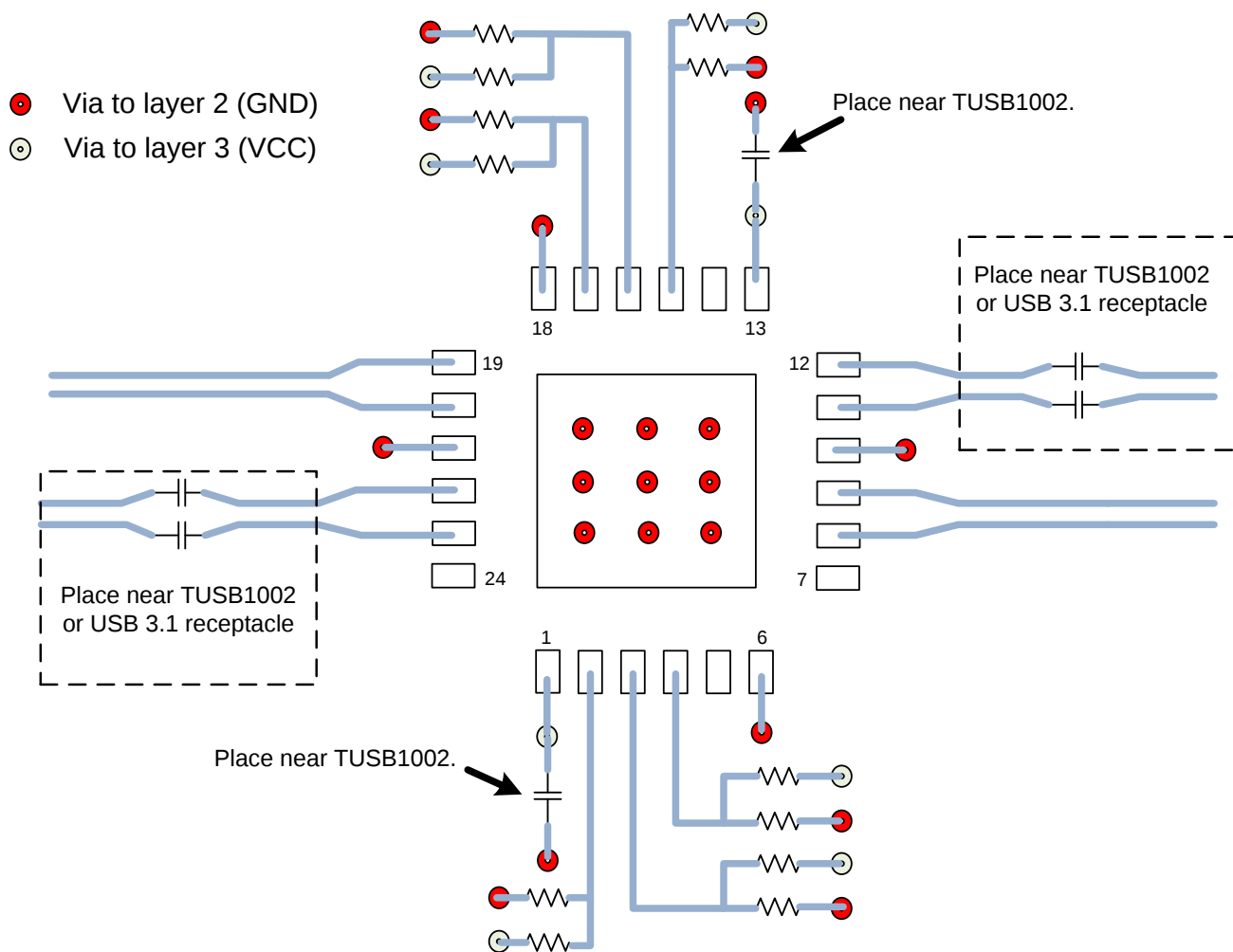
Figure 25. Example Layout
