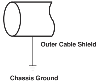
图 13-5. Non-DC-Isolated Outer Shield Termination
