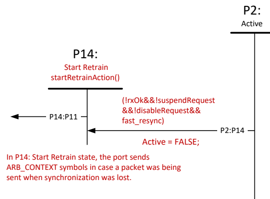
图 13-1. Fast-Retrain Port Connection State Machine Changes
