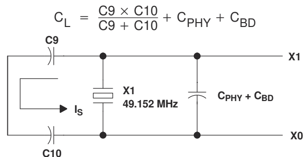
图 13-8. Load Capacitance for the TSB41BA3F-EP PHY
