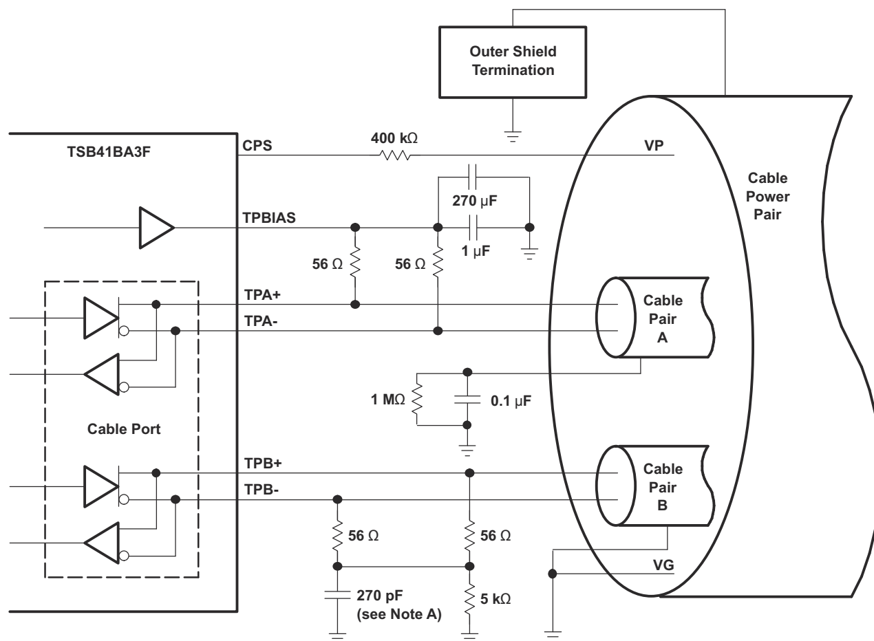
图 13-3. Typical TP Cable Connections
