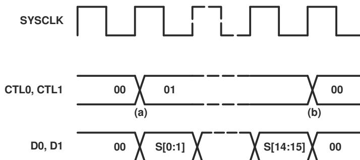
图 12-3. Status Transfer Timing
