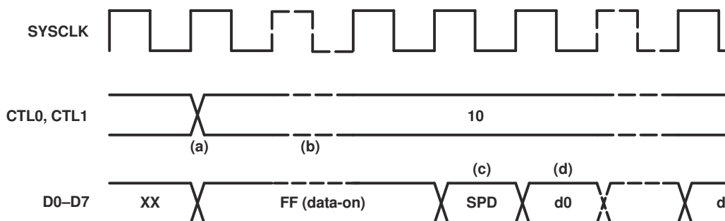
图 12-4. Normal Packet Reception Timing
