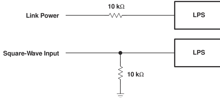
图 13-6. Nonisolated Connection Variations For LPS
