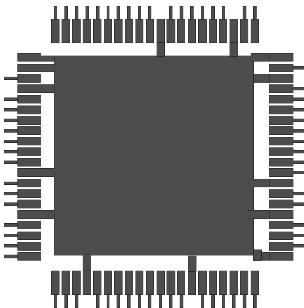
图 13-10. Example of a Thermal Land for the TSB41BA3F-EP PHY
