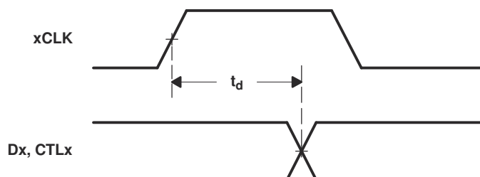
图 8-3. Dx and CTLx Output Delay Relative to xCLK Waveforms
