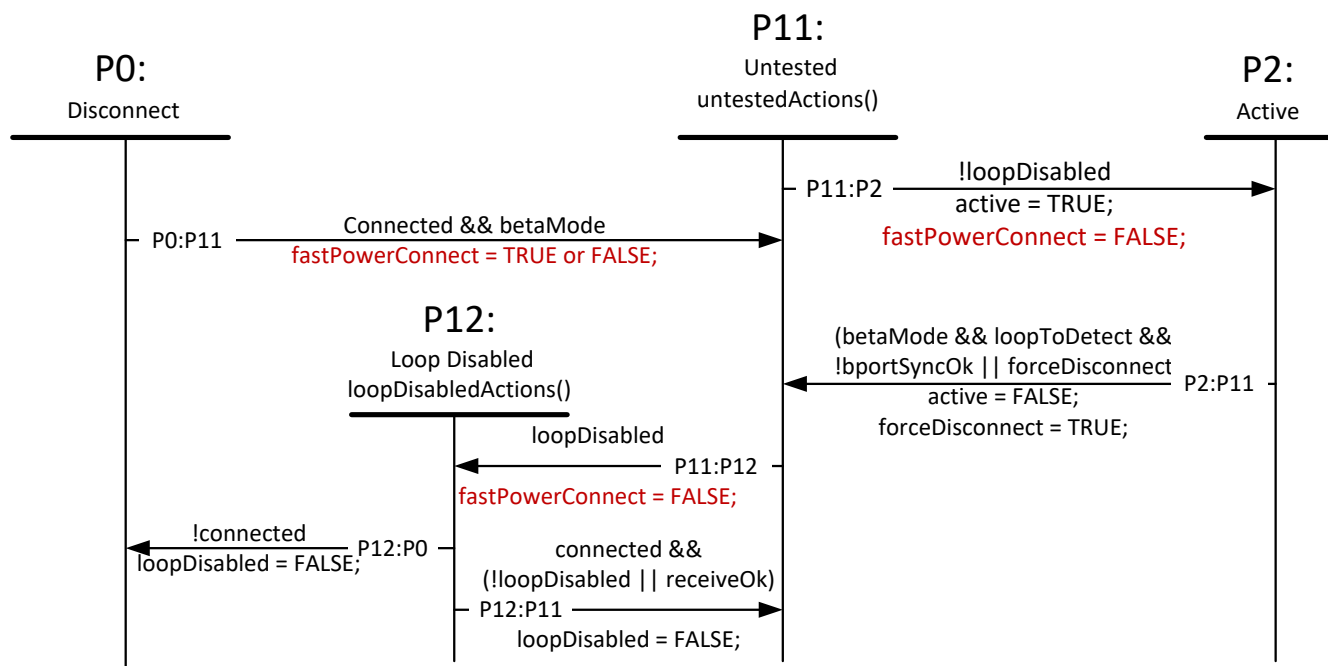
图 13-2. Fast Power-On Re-Connect Port Connection State Machine Changes
