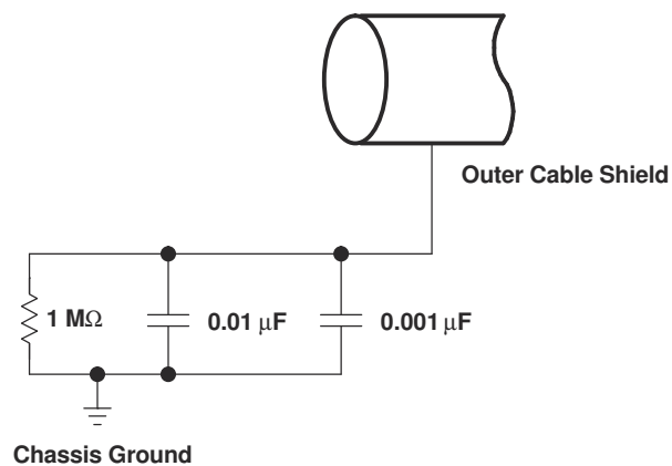
图 13-4. Typical DC-Isolated Outer Shield Termination
