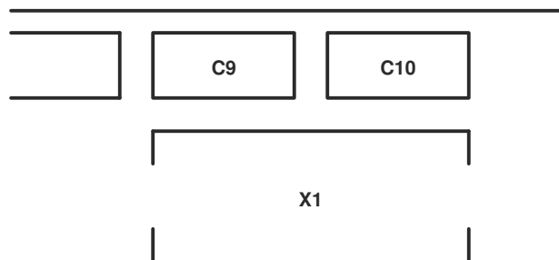
图 13-9. Recommended Crystal And Capacitor Layout
