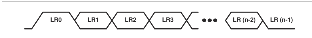
图 11-4. PINT (PHY Interrupt) Stream
