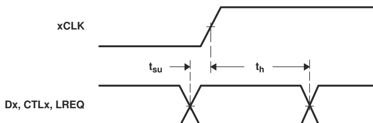
图 8-2. Dx, CTLx, LREQ Input Setup and Hold Time Waveforms
