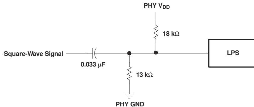
图 13-7. Isolated Circuit Connection For LPS
