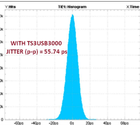
Figure 23. Time Interval Error Histogram: 2.2 Gbps for MHL Switch
