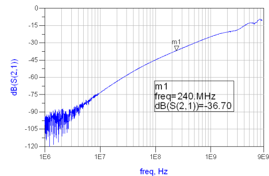
Figure 4. Differential S21 vs Frequency for MHL Switch
