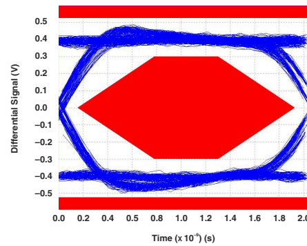
图 7-3. Eye Pattern: 480-Mbps USB Signal With Switch 1D Path
