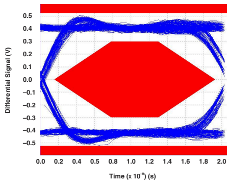
图 7-2. Eye Pattern: 480-Mbps USB Signal With No Switch (Through Path)
