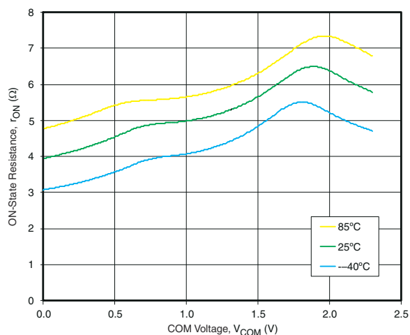
图 6-2. ON-State Resistance vs COM Voltage ( V_{CC} = 2.3\text{ V} )
