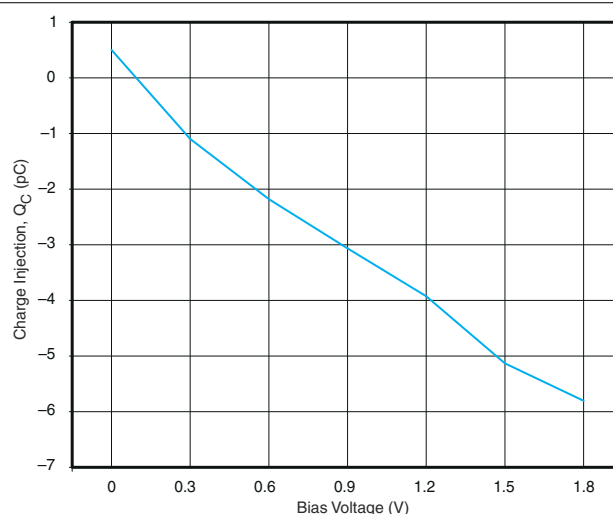
图 6-12. Charge Injection vs Bias Voltage (1.8 V)
