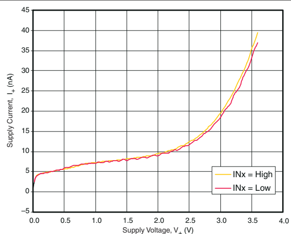
图 6-5. Supply Current vs Supply Voltage
