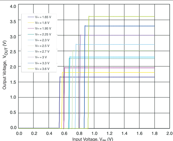
图 6-6. Control Input Thresholds (IN1, T_A = 25^\circ\text{C} )
