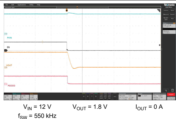
图 8-22. Shutdown from CNTL
