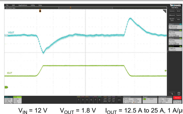
图 8-12. Load Transient Response
