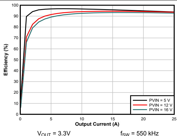
图 8-2. Efficiency vs Output Current
