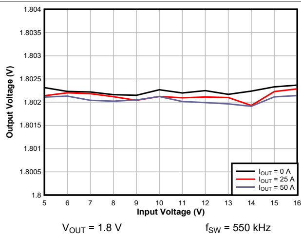
图 8-20. Line Regulation
