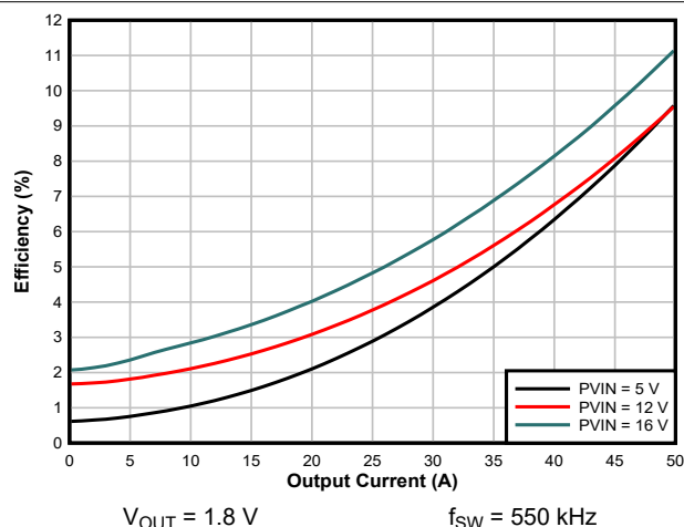
图 8-18. Power Dissipation vs Output Current
