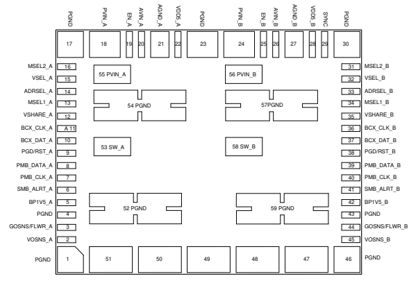
图 5-2. 59-Pin QFM-MOW Package (Bottom View)
