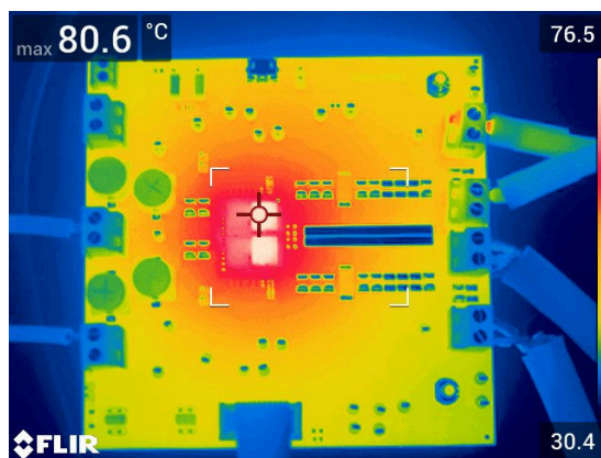
图 8-29. Thermal Image at 25°C Ambient, 12 V IN , Dual 1.0 V OUT , 25 A, 550 kHz
