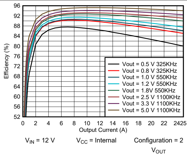
图 6-3. TPSM8D6B24 Efficiency vs Output Current
