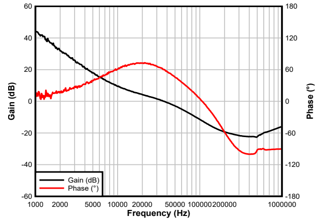
图 8-8. Total-Loop Bode Plot
