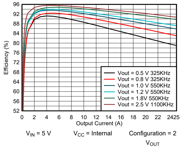
图 6-1. TPSM8D6B24 Efficiency vs Output Current
