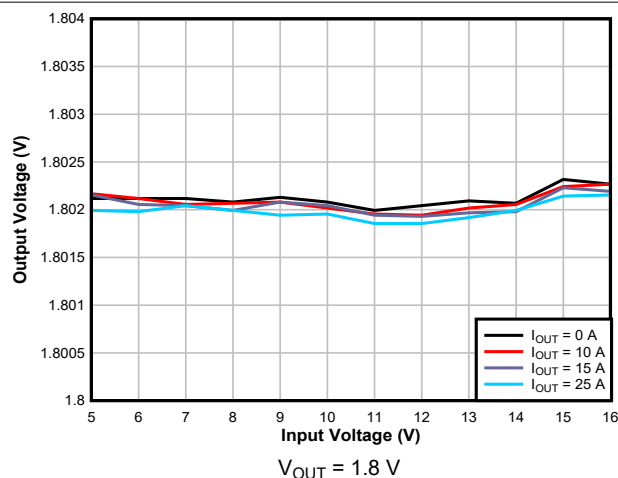
图 8-5. Line Regulation
