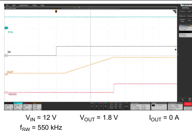
图 8-21. Start-Up from EN/UVLO
