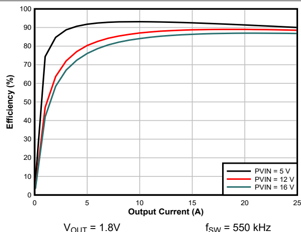
图 8-1. Efficiency vs Output Current
