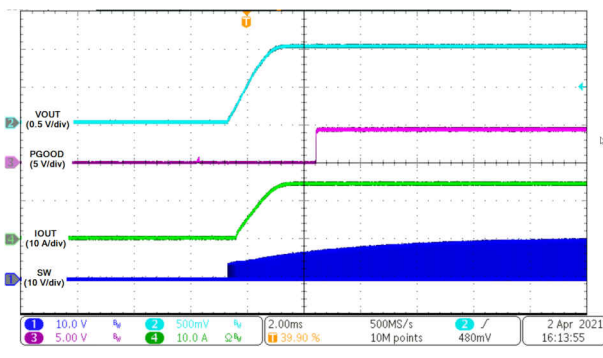
图 8-32. Startup Through V_{IN} (Enable Floating)
