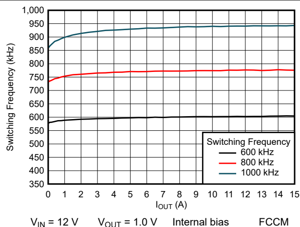
图 8-20. Switching Frequency
