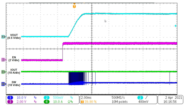
图 8-33. Startup Through Enable
