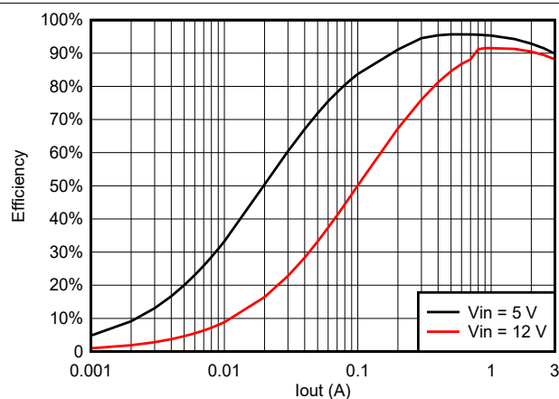
图 6-14. TPSM863253 Efficiency at 3.3V OUT
