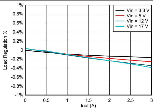
图 8-3. TPSM863257 Load Regulation vs Loading
