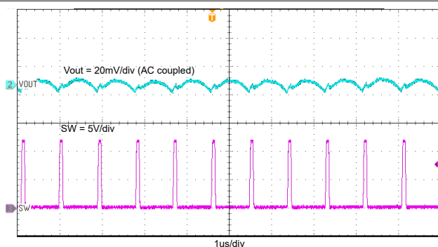
图 8-7. TPSM863257 Output Voltage Ripple With 0.01A Loading
