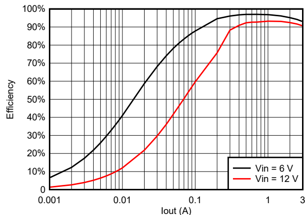
图 6-16. TPSM863257 Efficiency at 5V OUT
