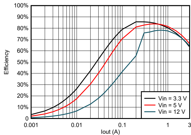
图 6-9. TPSM863257 Efficiency at 0.6V_{OUT}
