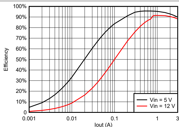
图 6-14. TPSM863253 Efficiency at 3.3V OUT
