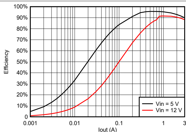
图 6-13. TPSM863257 Efficiency at 3.3V OUT
