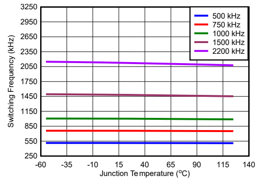
Figure 5-12. Switching Frequency
