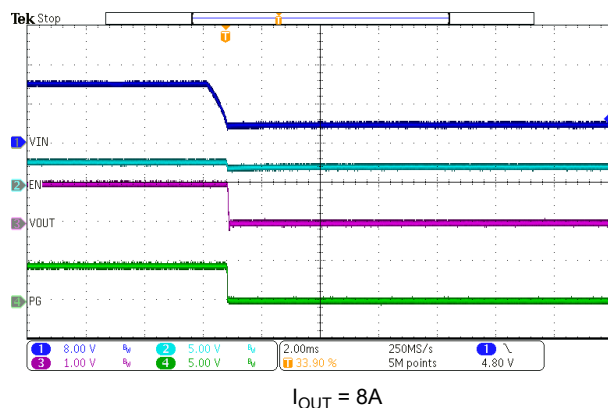
Figure 7-14. VIN Shutdown
