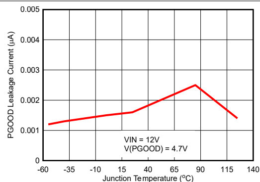
Figure 5-10. PG Leakage
