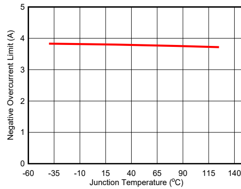
图 5-15. Negative Overcurrent
