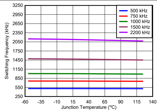
图 5-12. Switching Frequency
