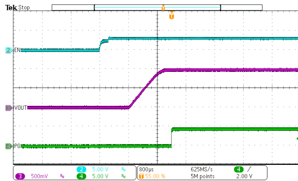
V_{IN} = 12V I_{OUT} = 6A 图 7-11. EN Start-Up – With Load
