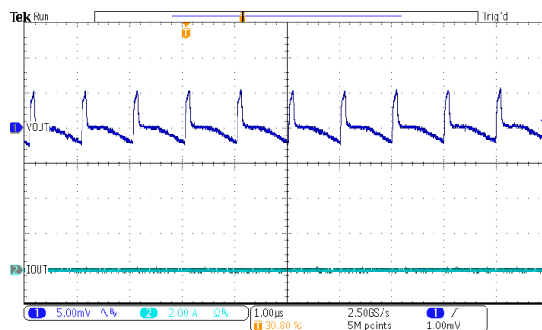
V_{IN} = 12V I_{OUT} = 0A 图 7-15. Output Ripple – No Load
