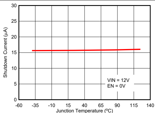
图 5-13. Shutdown Current
