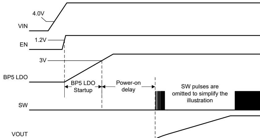
图 6-1. Start-Up Sequence
