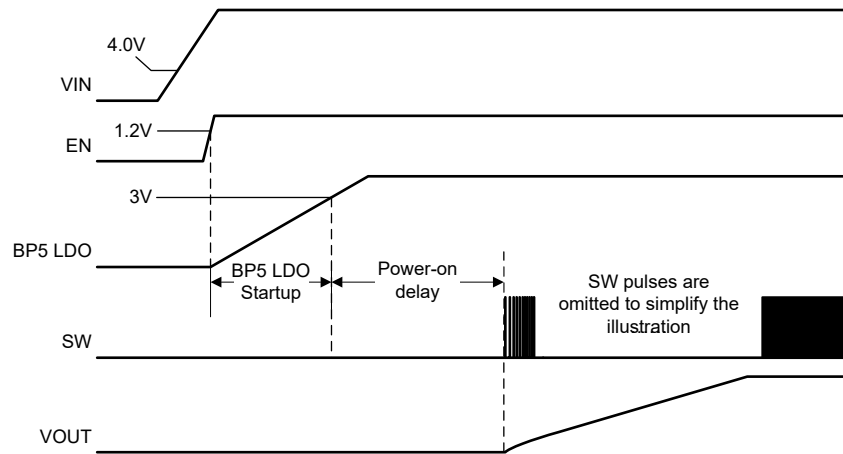
图 6-1. Start-Up Sequence
