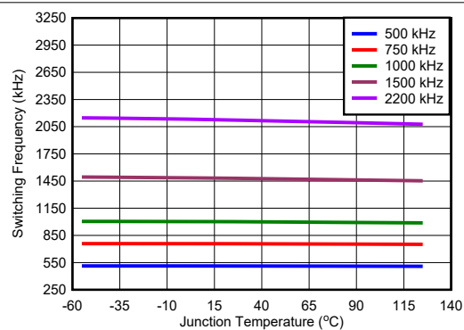
图 5-12. Switching Frequency
