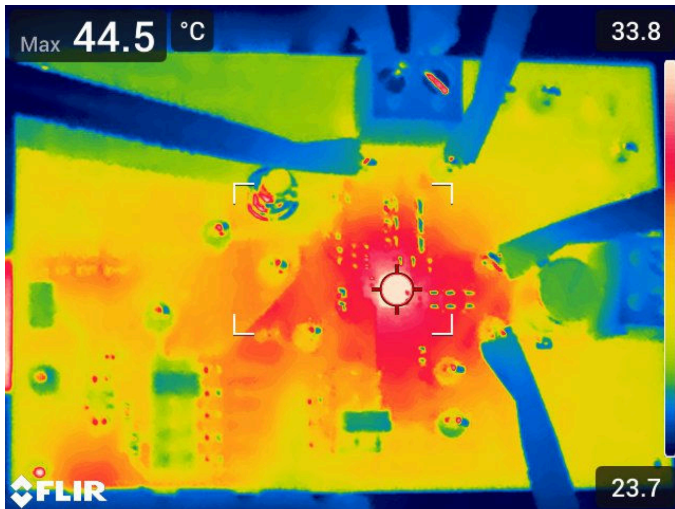
图 7-20. Thermal Image at 25^{\circ}\text{C} Ambient
