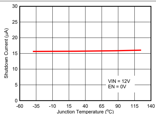
图 5-13. Shutdown Current
