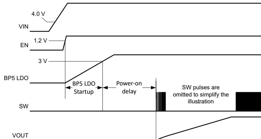
图 6-1. Start-Up Sequence
