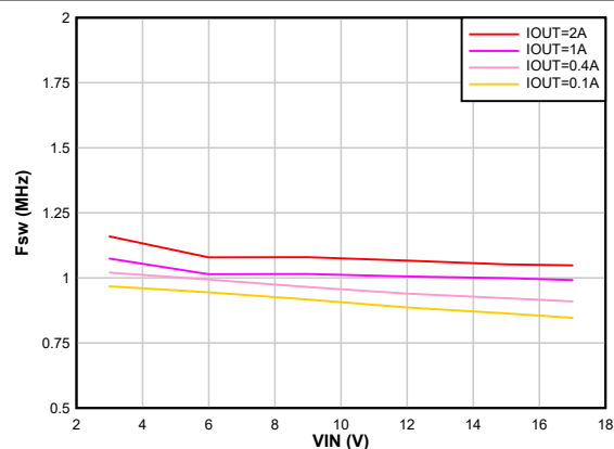
图 8-17. Switching Frequency vs Input Voltage V_{OUT} = 1.2 V
