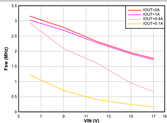
图 8-19. Switching Frequency vs Input Voltage V_{OUT} = 1.8 V
