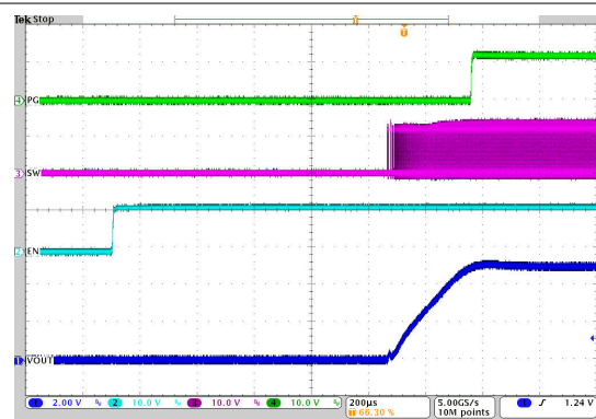
图 8-26. Start-Up Timing
