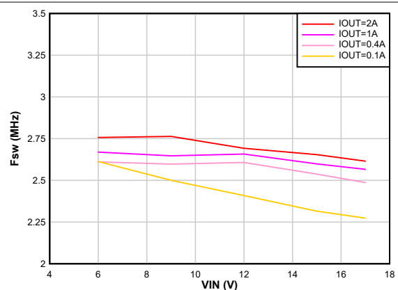
图 8-20. Switching Frequency vs Input Voltage V_{OUT} = 1.2 V
