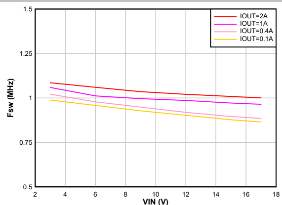
图 8-18. Switching Frequency vs Input Voltage V_{OUT} = 1.8 V
