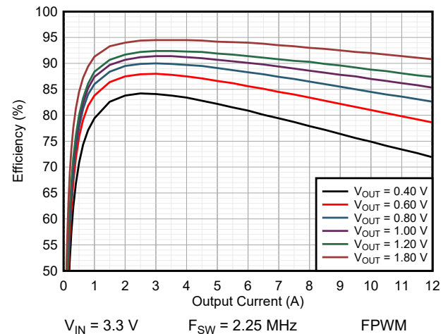
图 9-11. Efficiency TPSM8287A12BBS
