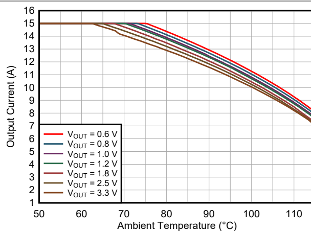
图 9-49. Safe Operating Area TPSM8287A15BBH V_{IN} = 5.0\text{ V}
