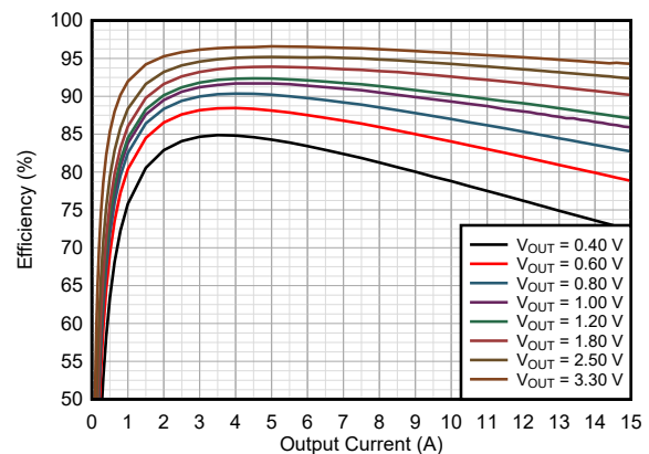
效率 TPSM8287A15BAH ( V_{IN} = 5.0\text{V} ; FPWM )
