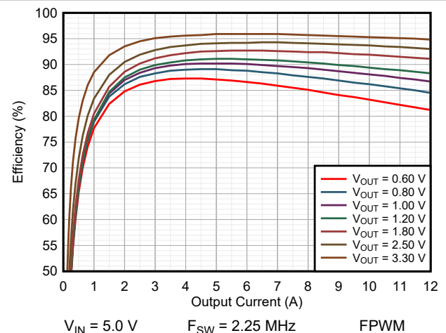
图 9-13. Efficiency TPSM8287A12BBS
