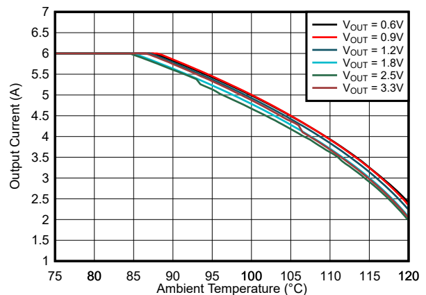
图 8-39. Safe Operating Area V_{IN} = 5.0\text{-V} TPSM82866AA0PRCFR
