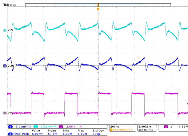
V_{IN} = 3.3\text{ V} V_{OUT} = 1.2\text{ V} C_{OUT} = 1 \times 47\mu\text{F} 图 8-28. FPWM Operation I_{OUT} = 3\text{ A}
