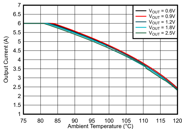
图 8-38. Safe Operating Area V_{IN} = 3.3\text{-V} TPSM82866AA0PRCFR
