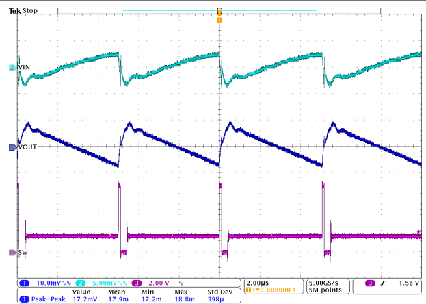
V_{IN} = 5.0\text{ V} V_{OUT} = 1.2\text{ V} C_{OUT} = 1 \times 47\mu\text{F} 图 8-29. PSM Operation I_{OUT} = 0.1\text{ A}
