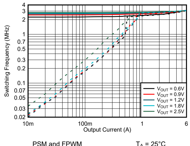
图 8-27. Switching Frequency V_{IN} = 3.3\text{ V}
