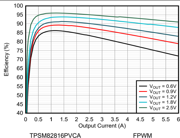
图 8-10. Efficiency V_{IN} = 3.3\text{ V} and T_A = 85^\circ\text{C}
