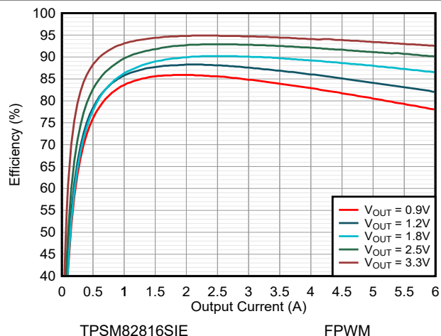
图 8-9. Efficiency V_{IN} = 5.0\text{ V} and T_A = 85^\circ\text{C}
