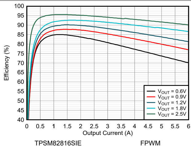
图 8-11. Efficiency V_{IN} = 3.3\text{ V} and T_A = 85^\circ\text{C}
