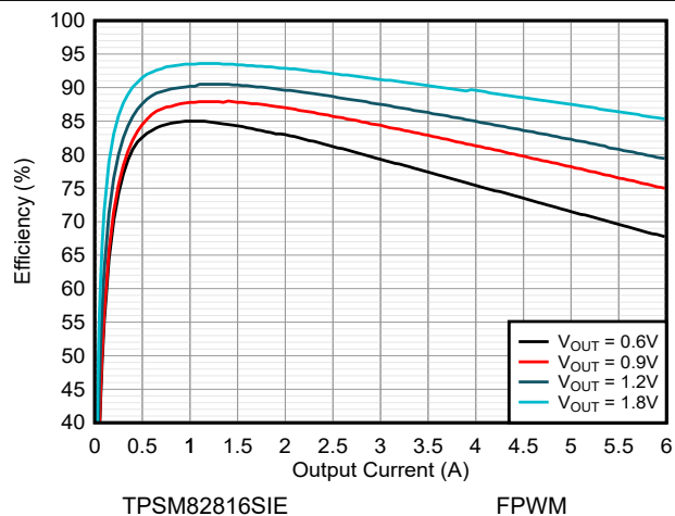
图 8-13. Efficiency V_{IN} = 2.7\text{ V} and T_A = 85^\circ\text{C}
