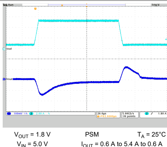
图 8-24. Load Transient Response
