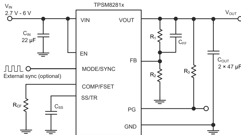
图 8-35. Frequency Synchronization
