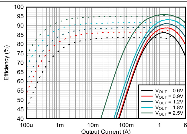
TPSM82816SIE PSM and FPWM
