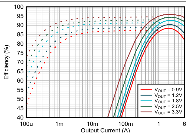
TPSM82816PVCA PSM and FPWM
