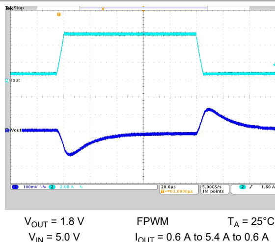
图 8-25. Load Transient Response
