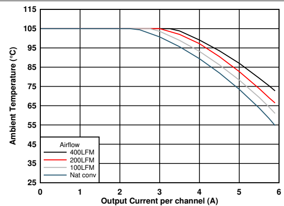
图 6-4. Safe Operating Area (VOUT = 1.2 V)
