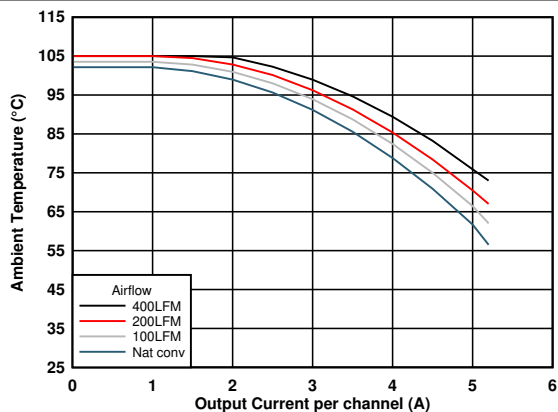
图 6-7. Safe Operating Area (VOUT = 5 V)
