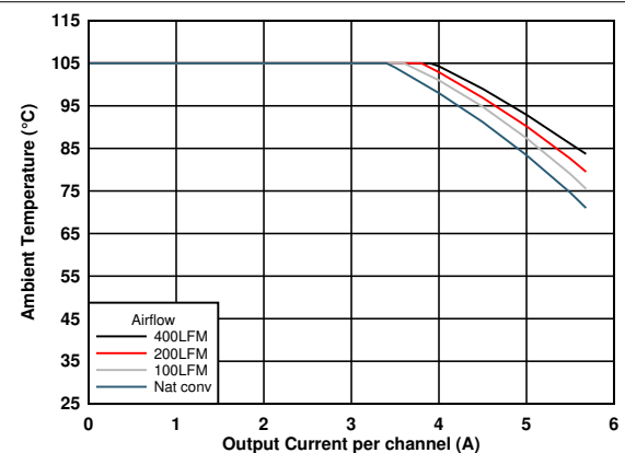
图 6-11. Safe Operating Area (VOUT = 0.8 V)
