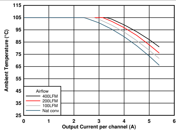
图 6-14. Safe Operating Area (VOUT = 3.3 V)
