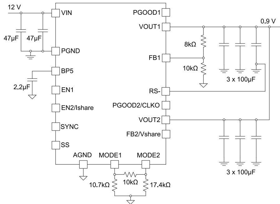
图 8-2. TPSM5D1806 Parallel Outputs Typical Schematic
