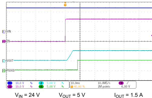
图 9-2. Start-up Waveforms
