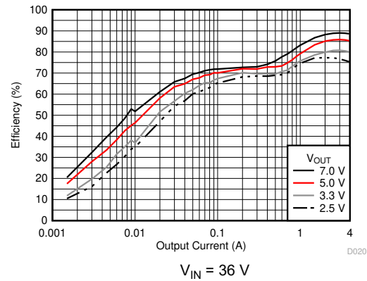
图 6-20. Efficiency versus Output Current
