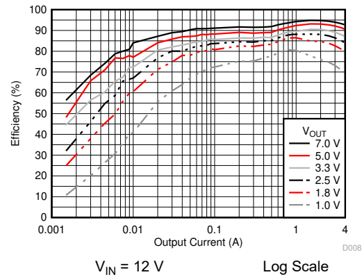
图 6-8. Efficiency versus Output Current
