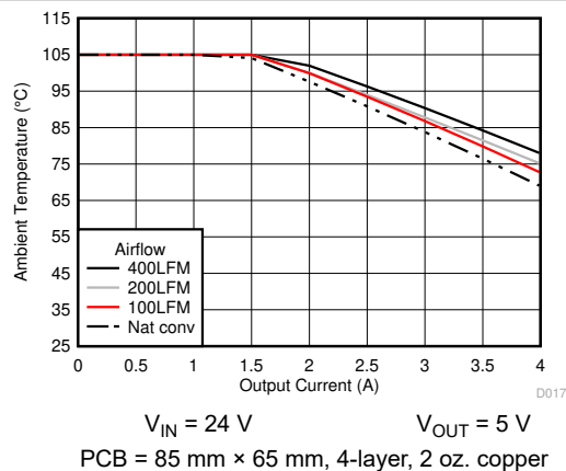
图 6-18. Safe Operating Area
