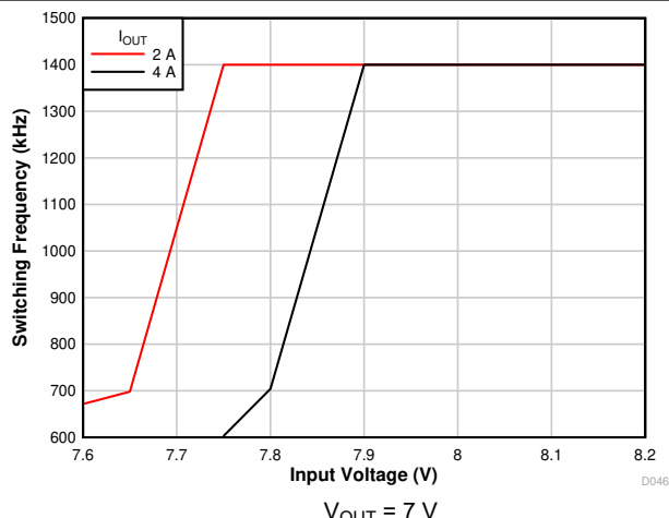
图 7-12. Frequency Foldback
