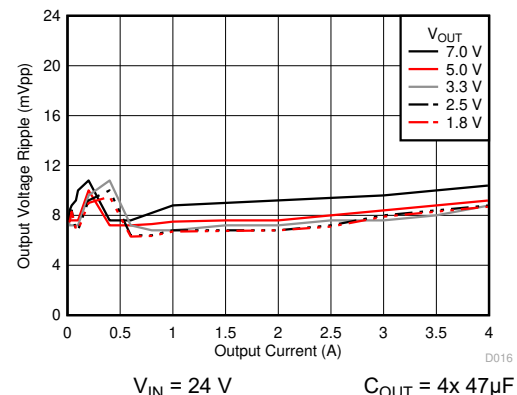
图 6-16. Voltage Ripple versus Output Current
