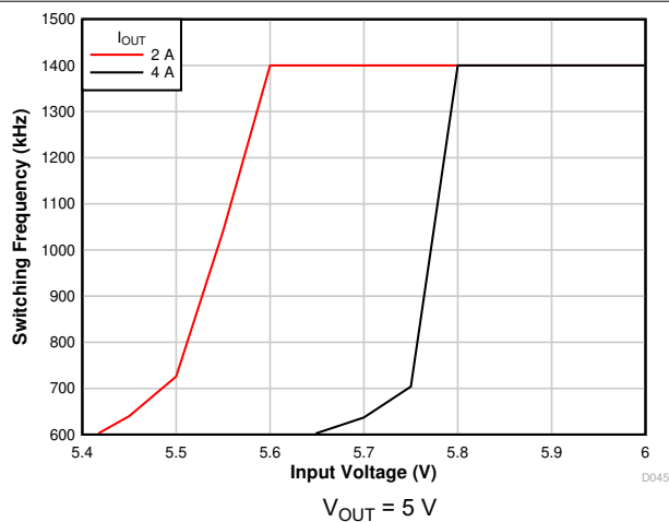
图 7-10. Frequency Foldback
