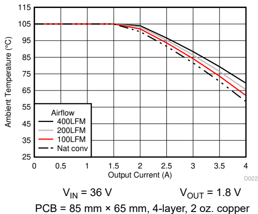
图 6-23. Safe Operating Area
