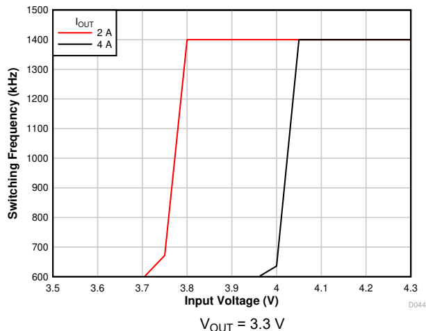
图 7-8. Frequency Foldback
