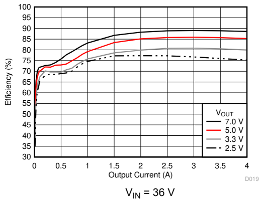
图 6-19. Efficiency versus Output Current
