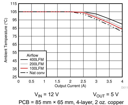
图 6-12. Safe Operating Area
