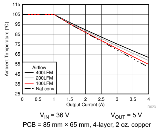
图 6-24. Safe Operating Area
