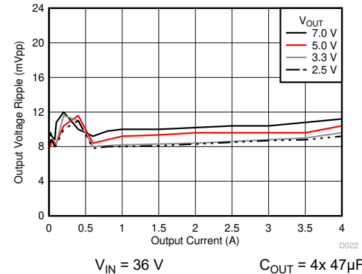
图 6-22. Voltage Ripple versus Output Current
