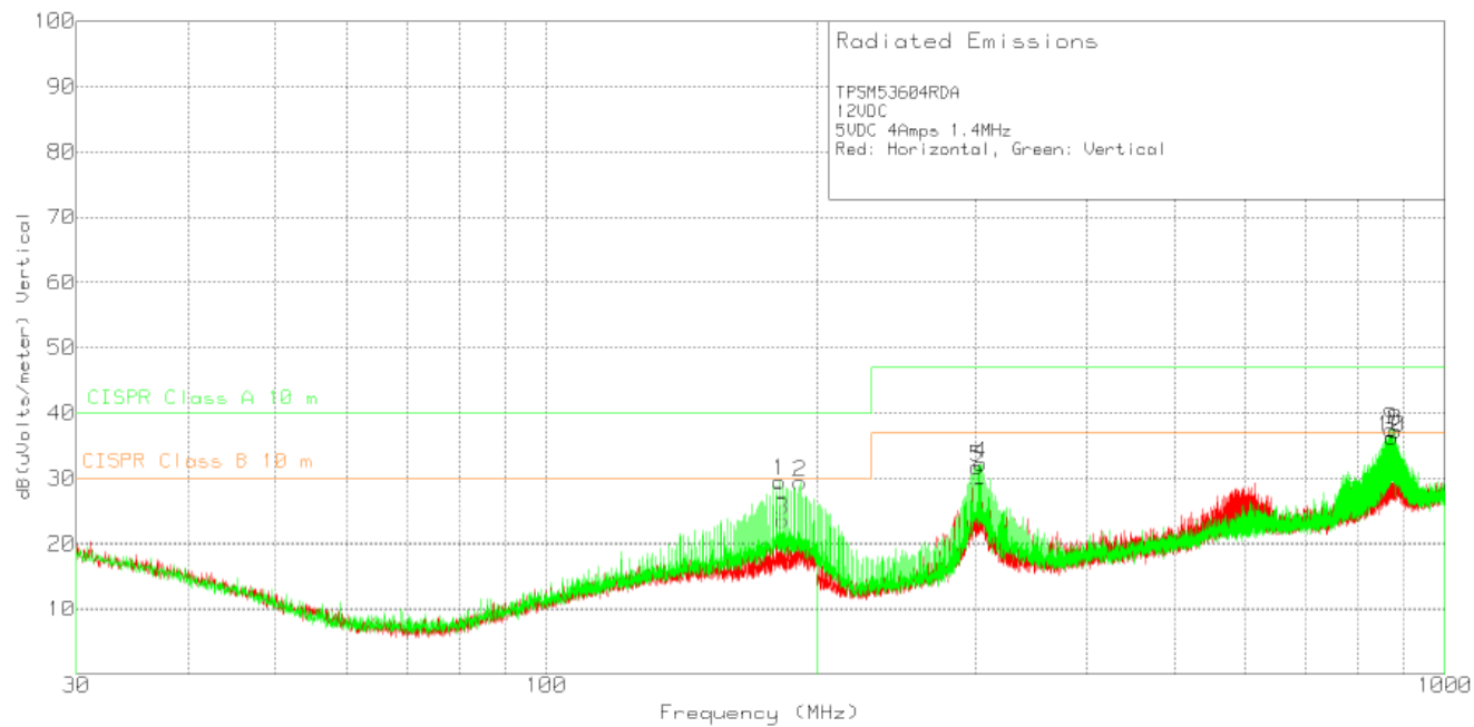
图 10-6. Radiated Emissions 12-V Input, 5-V Output, 4-A Load
