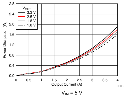
图 6-3. Power Dissipation versus Output Current
