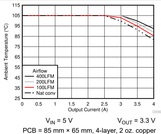
图 6-6. Safe Operating Area
