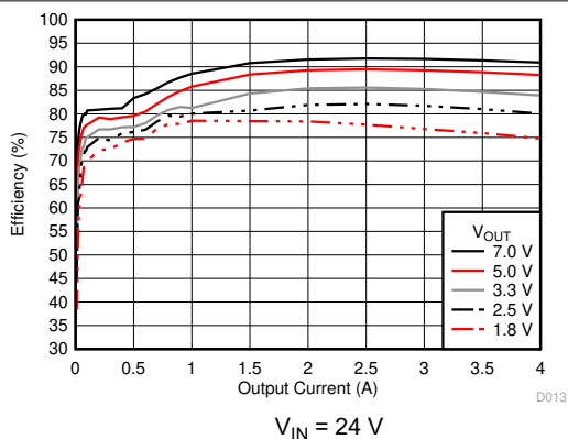
图 6-13. Efficiency versus Output Current
