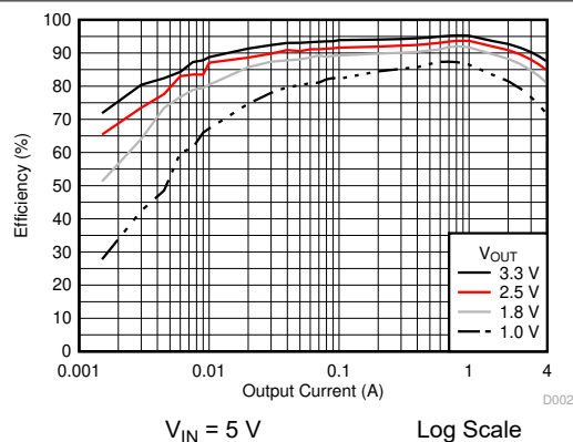
图 6-2. Efficiency versus Output Current
