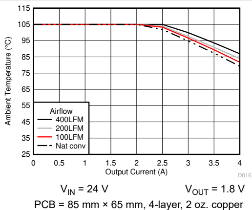
图 6-17. Safe Operating Area
