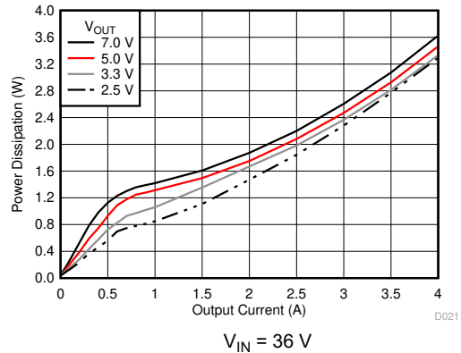
图 6-21. Power Dissipation versus Output Current
