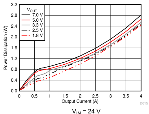
图 6-15. Power Dissipation versus Output Current
