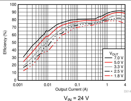
图 6-14. Efficiency versus Output Current
