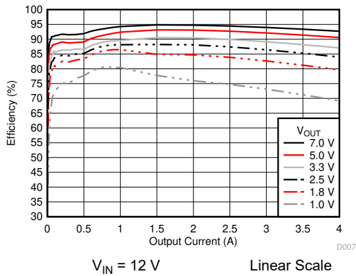
图 6-7. Efficiency versus Output Current
