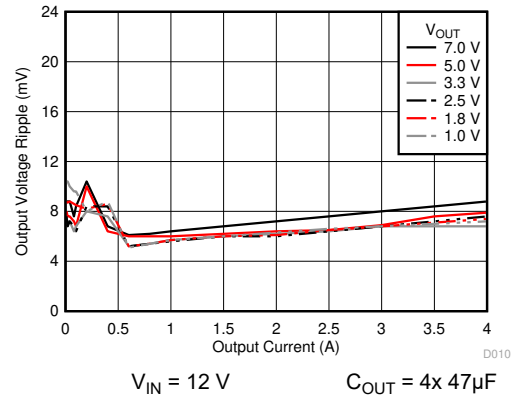
图 6-10. Voltage Ripple versus Output Current
