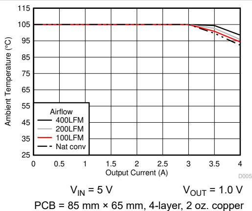
图 6-5. Safe Operating Area
