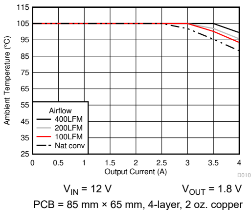
图 6-11. Safe Operating Area
