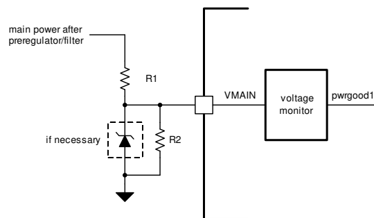
图 6-29. VMAIN Brown Out Monitor
