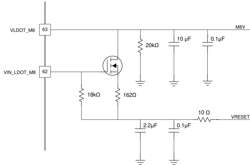
图 6-32. Negative 8V LDO Circuit
