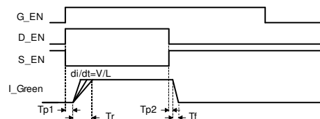
图 6-7. First Generation/Legacy System Pulse Distortion Example
