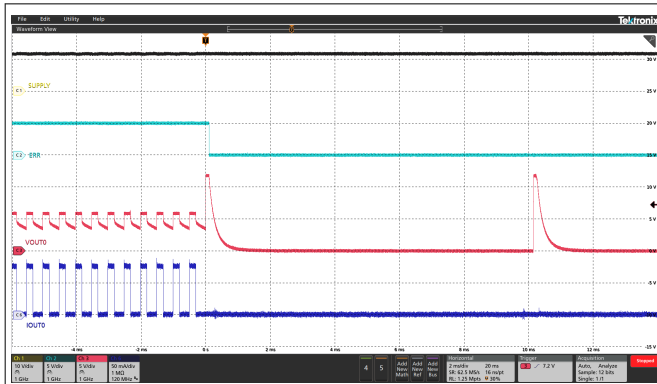
图 6-25. LED Open-Circuit Detection In FS Mode
