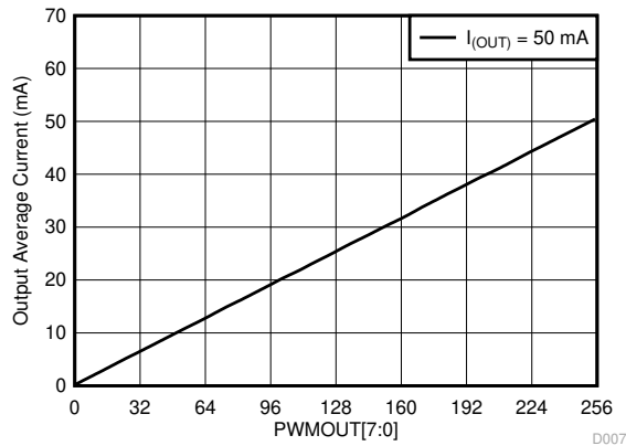
图 6-7. Average Current vs PWMOUT[7:0]
