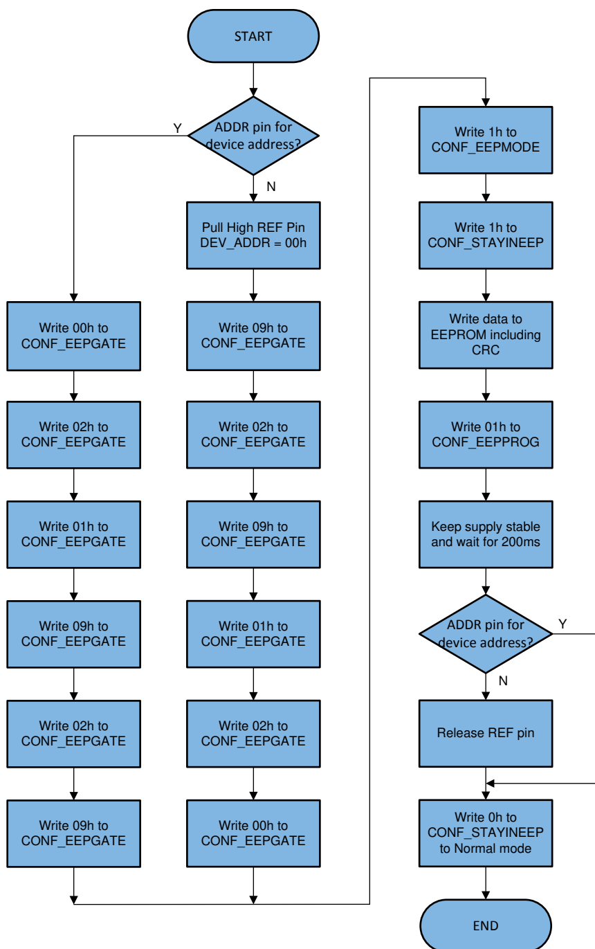
图 7-18. Programming Sequence
