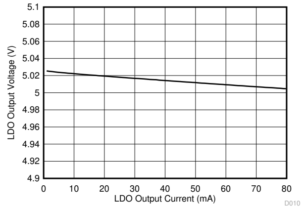
图 6-10. LDO Output Load Regulation
