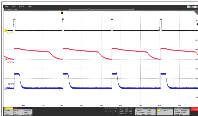
图 6-13. Supply Dimming In Fail-Safe Mode
