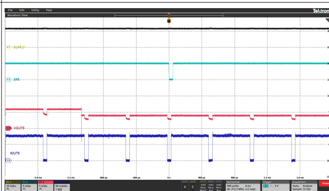
图 6-22. LED Open-Circuit Detection In Normal Mode
