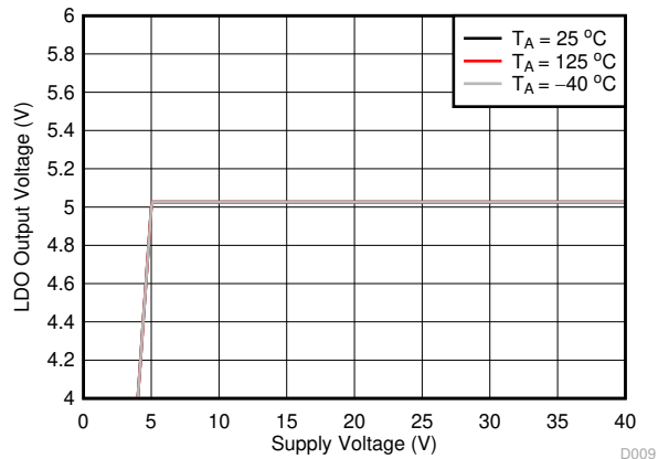
图 6-9. LDO Output Line Regulation
