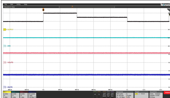
图 6-13. Supply Dimming In Fail-Safe Mode
