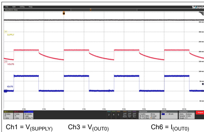
图 6-11. PWM Dimming at 200 Hz
