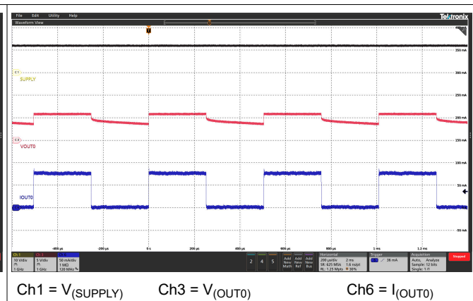
图 6-12. PWM Dimming at 2000 Hz
