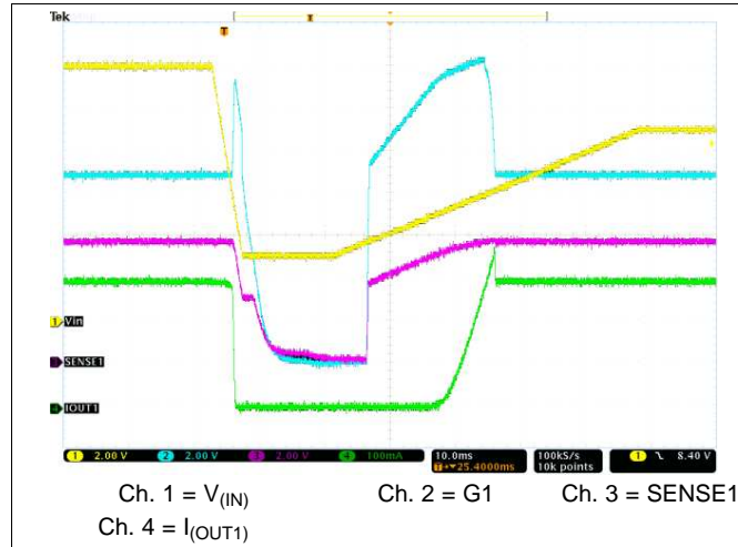
图 14. Fast Power Down and Slow Power Up
