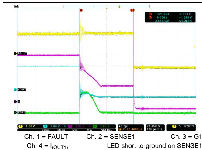
图 18. LED Hard Short Protection and One-Fails-All-Fail
