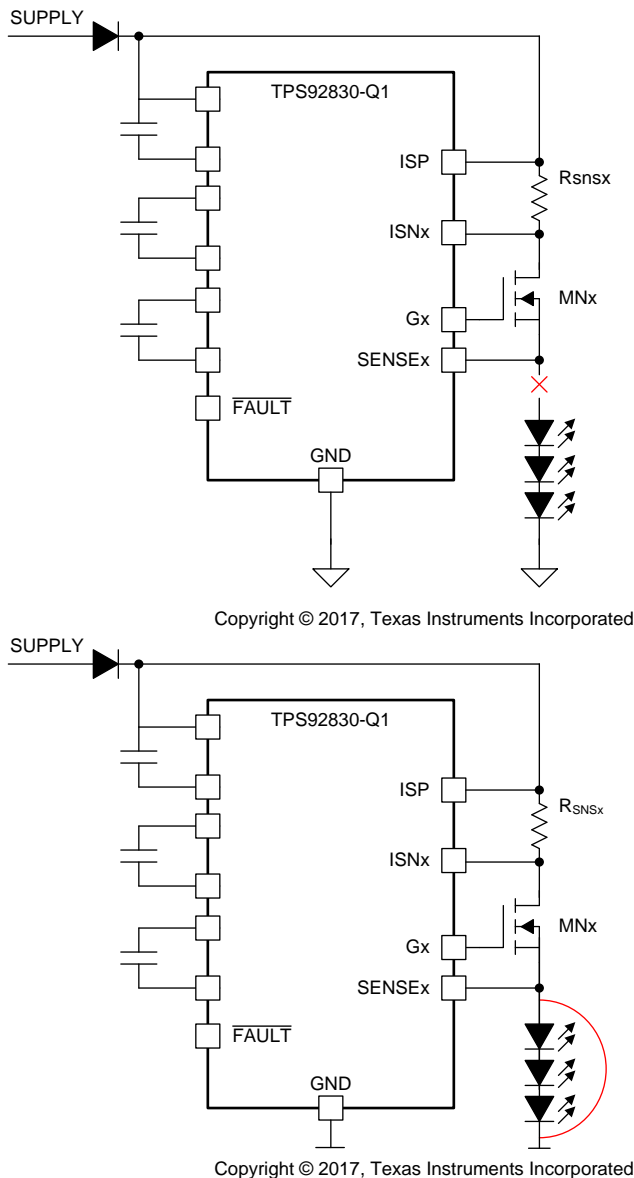
图 29. LED Open and Short Scenarios
