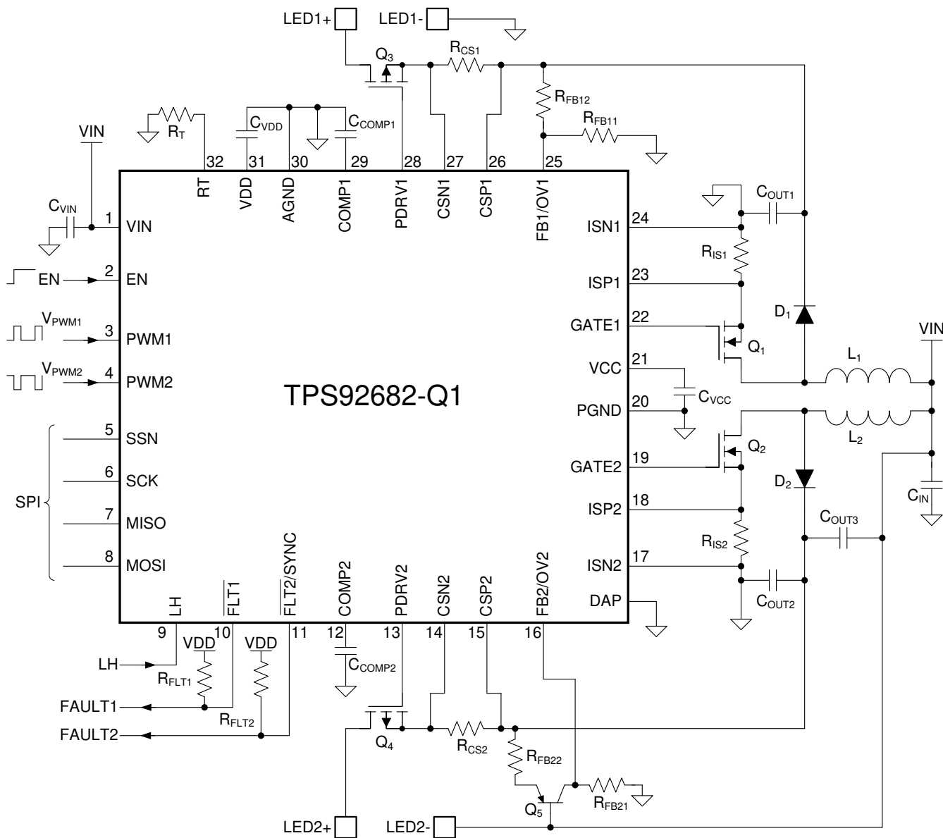
图 8-2. Two-Channel LED Driver, BOOST, and BUCK-BOOST Topology (CC mode)
