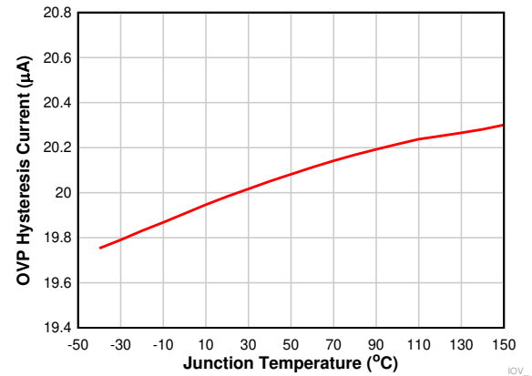
图 6-14. OVP Hysteresis Current vs Junction Temperature
