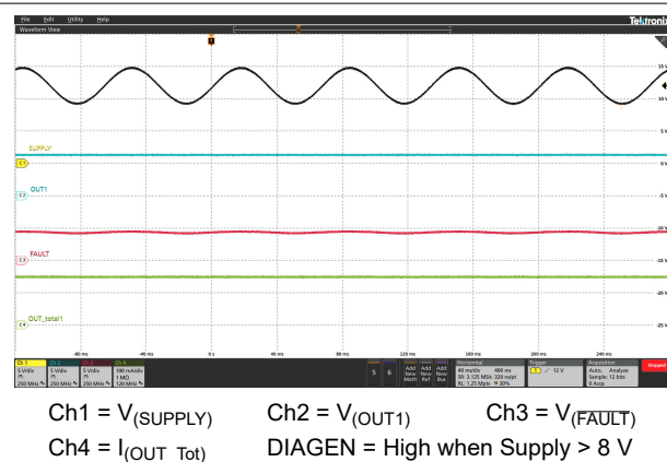
图 6-22. Superimposed Alternating Voltage 15 Hz
