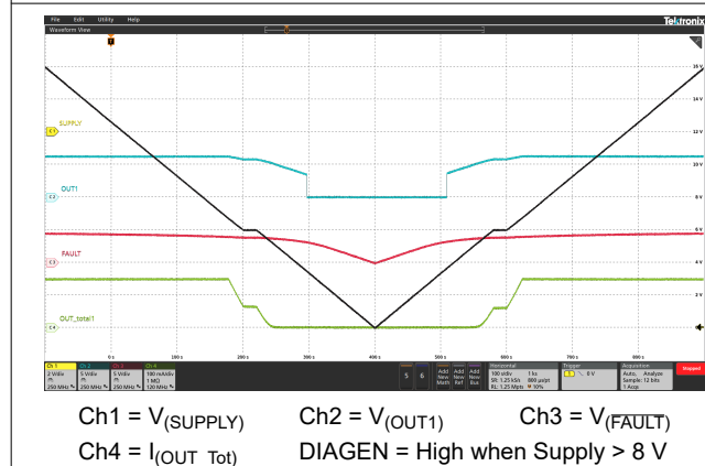
图 6-21. Slow Decrease and Slow Increase of Supply Voltage
