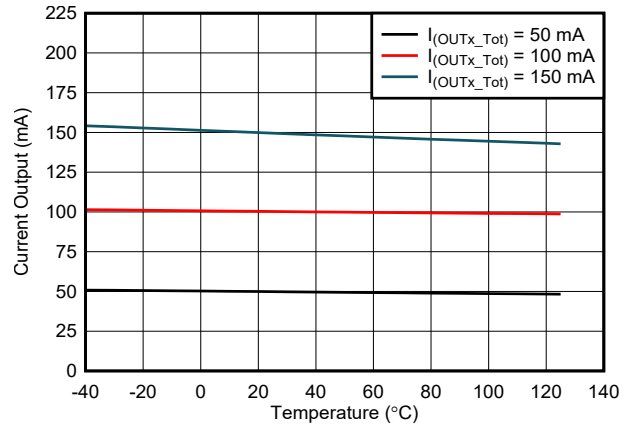
图 6-2. Output Current vs Temperature
