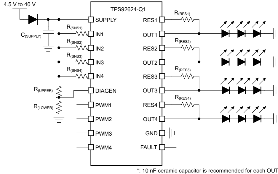
图 7-5. Application Schematic For DIAGEN
