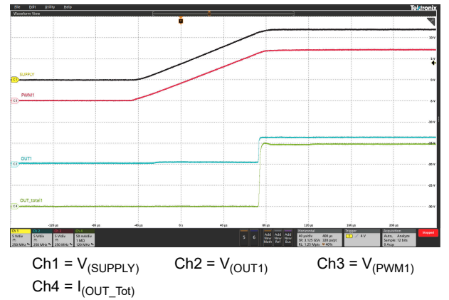
图 6-10. Power Up Sequence
