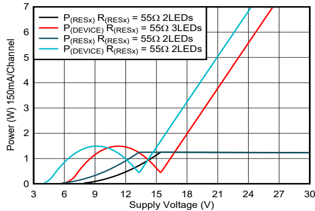
图 6-9. Power Dissipation vs Supply Voltage
