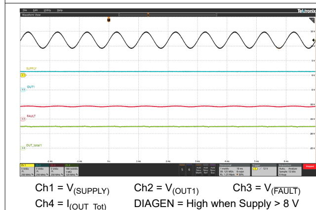
图 6-23. Superimposed Alternating Voltage 1 kHz
