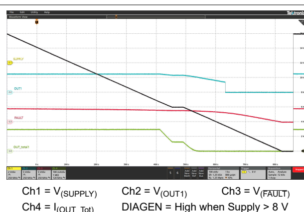
图 6-20. Slow Decrease and Quick Increase of Supply Voltage
