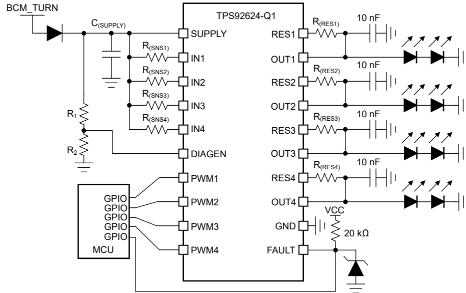
图 8-4. Typical Application Schematic
