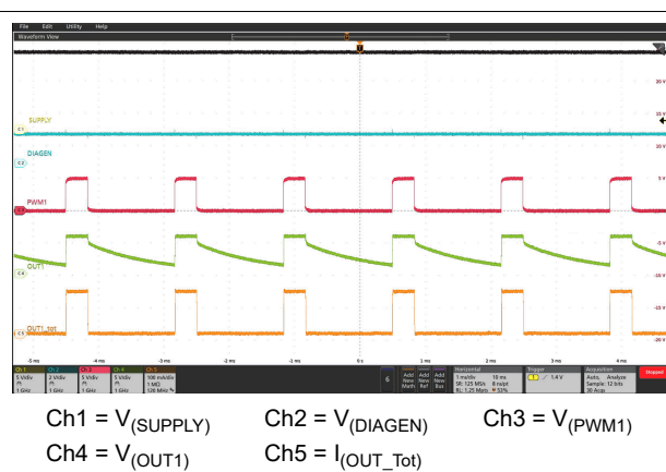
图 8-6. 600-Hz PWM Dimming at 20% Duty Cycle
