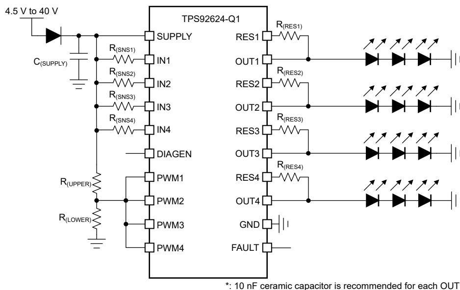
图 7-2. Application Schematic for Supply Control LED Brightness
