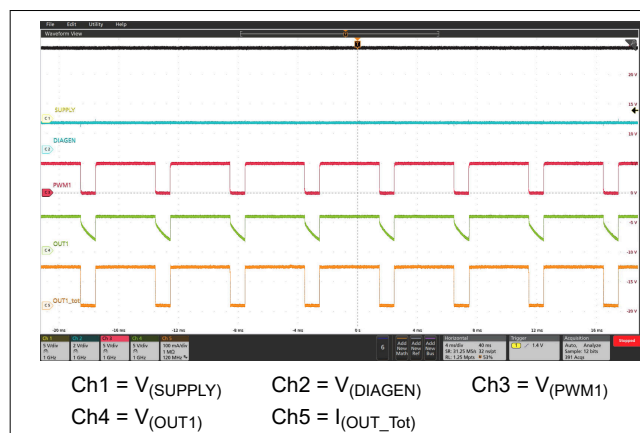
图 8-5. 200-Hz PWM Dimming at 80% Duty Cycle
