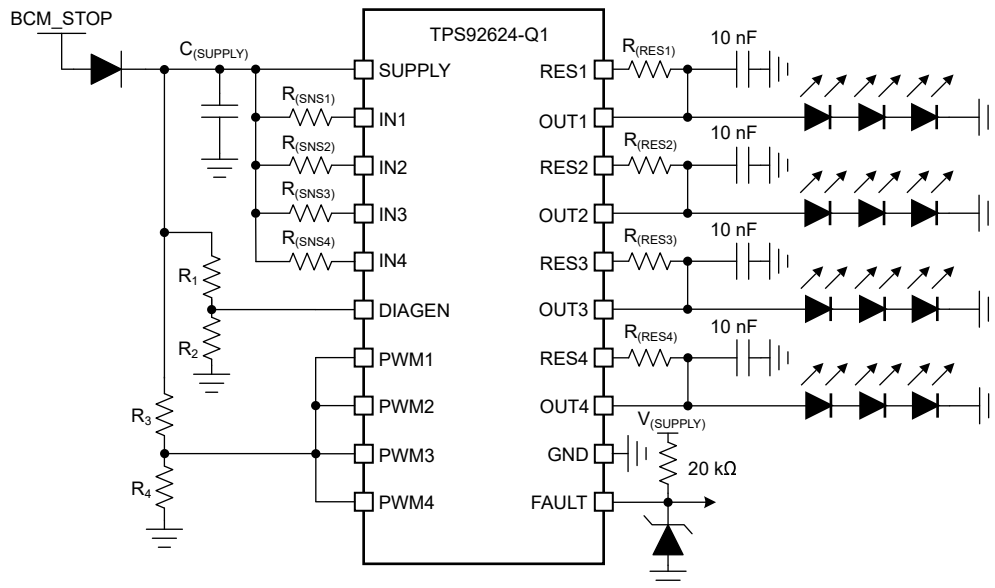
图 8-1. Typical Application Schematic
