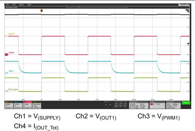
图 6-12. PWM Dimming at 200 Hz
