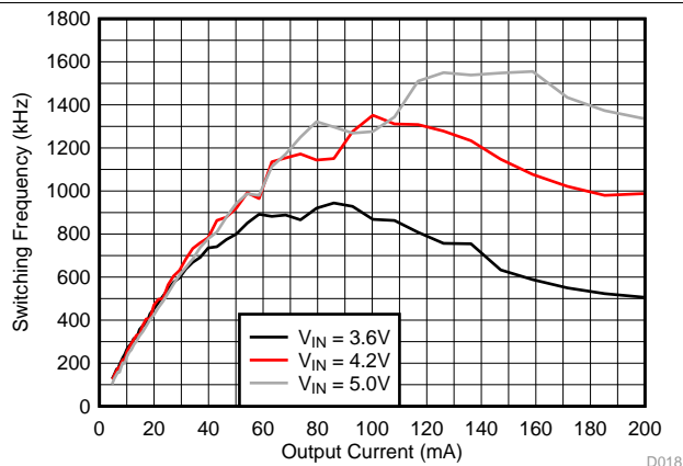
Figure 15. TPS82740A Switching frequency V_{OUT} = 1.8V
