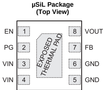
Pin Functions
