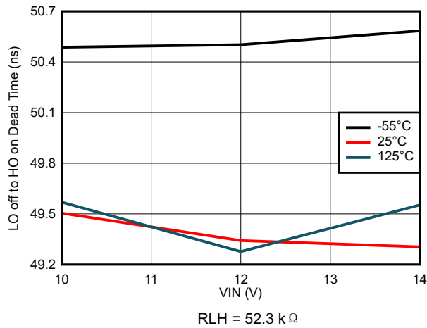
图 7-33. LO off to HO on Dead Time vs VIN Voltage
