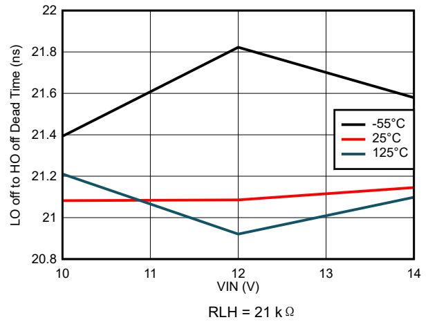
图 7-32. LO off to HO on Dead Time vs VIN Voltage
