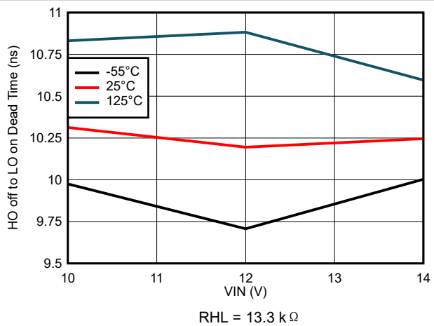
图 7-36. HO off to LO on Dead Time vs VIN Voltage
