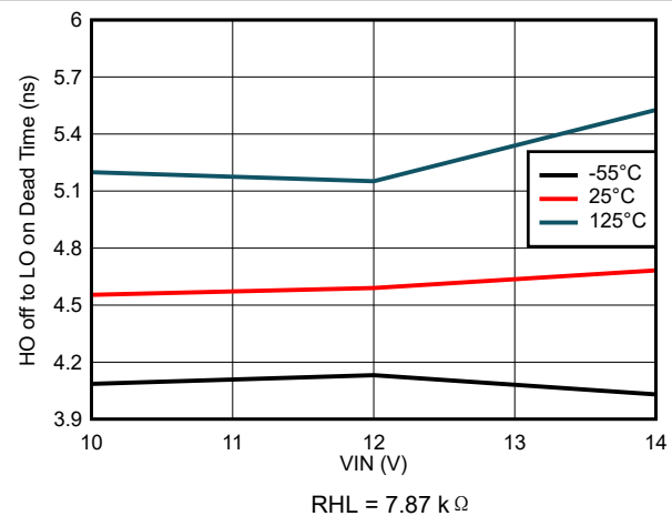
图 7-35. HO off to LO on Dead Time vs VIN Voltage
