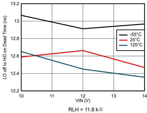
图 7-31. LO off to HO on Dead Time vs VIN Voltage
