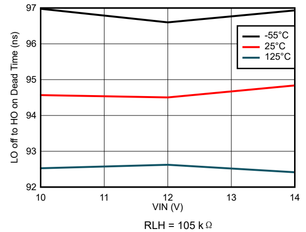
图 7-34. LO off to HO on Dead Time vs VIN Voltage
