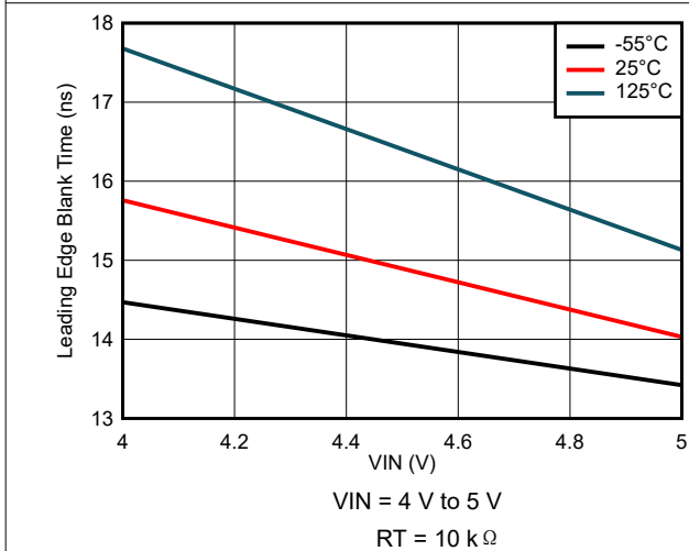
图 7-33. Leading Edge Blank Time Variation
