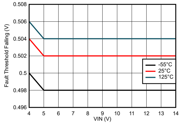
图 7-32. FAULT Threshold Falling Variation
