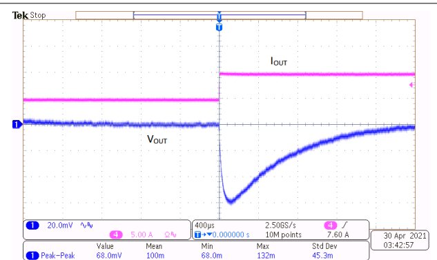
图 9-3. 5-A Load Step Response for Push Pull Converter
