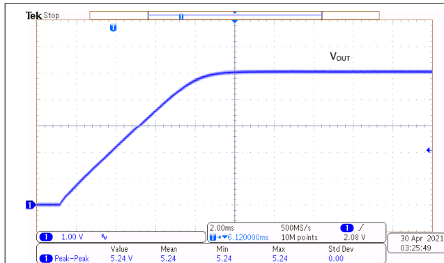
图 9-2. V_{OUT} Soft-Start of Push-Pull Converter With I_{OUT} = 10 \text{ A}
