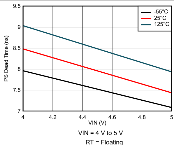
图 7-41. PS Dead Time Variation
