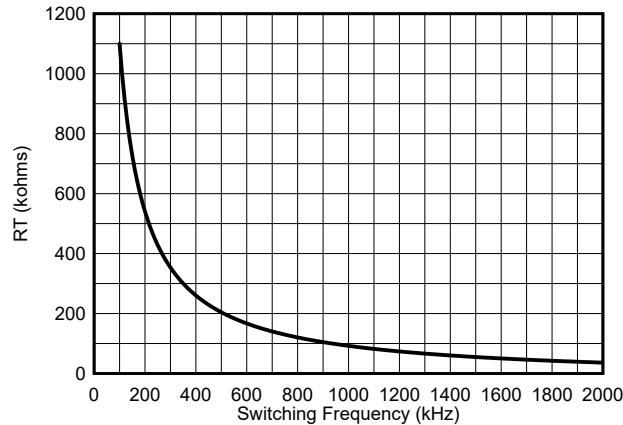
图 8-7. RT vs Switching Frequency
