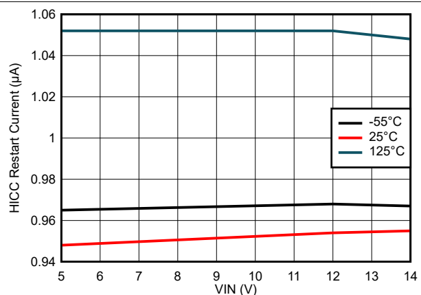
图 7-28. Hiccup Delay Current Variation
