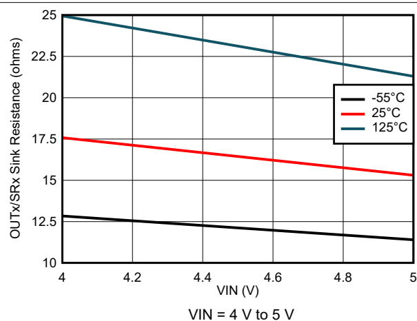
图 8-63. Output Sink Resistance Variation
