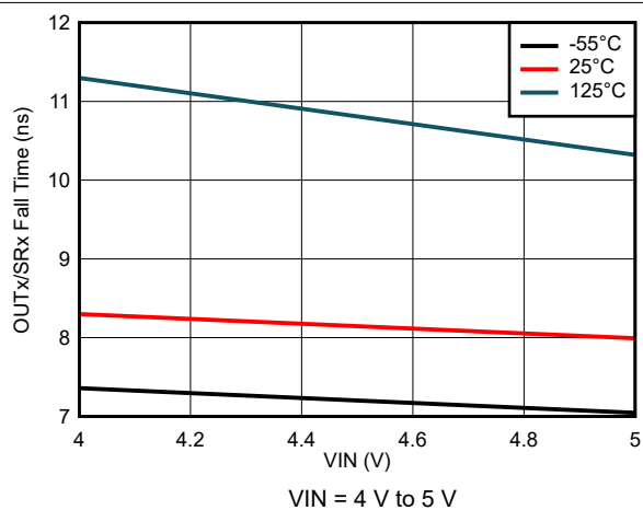
图 8-59. Output Fall Time Variation
