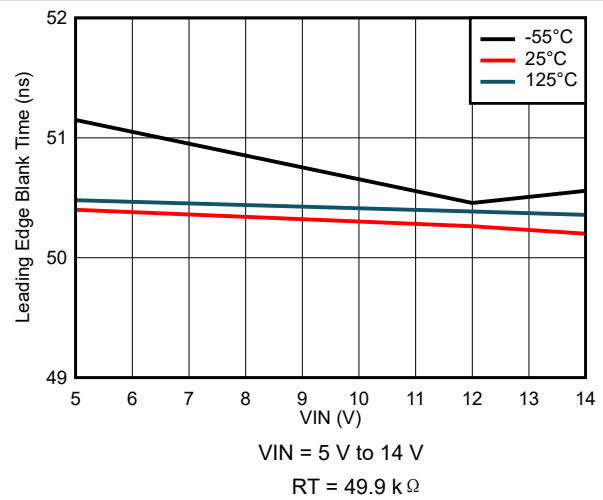
图 8-36. Leading Edge Blank Time Variation
