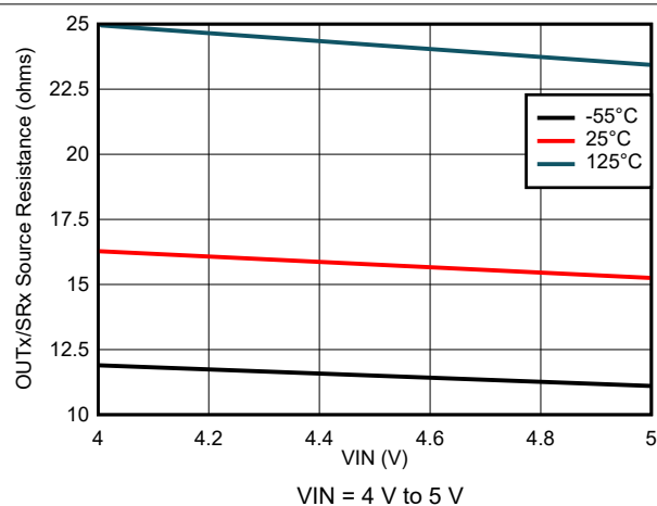
图 8-61. Output Source Resistance Variation
