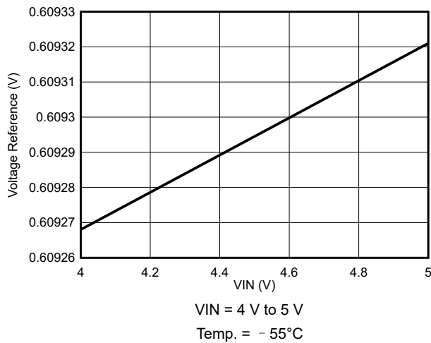
图 8-11. Voltage Reference Variation
