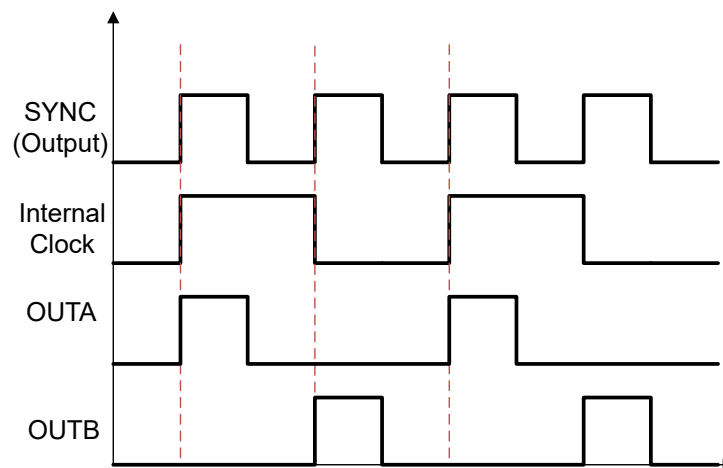
图 9-8. Switching Waveforms for Internal Oscillator Mode
