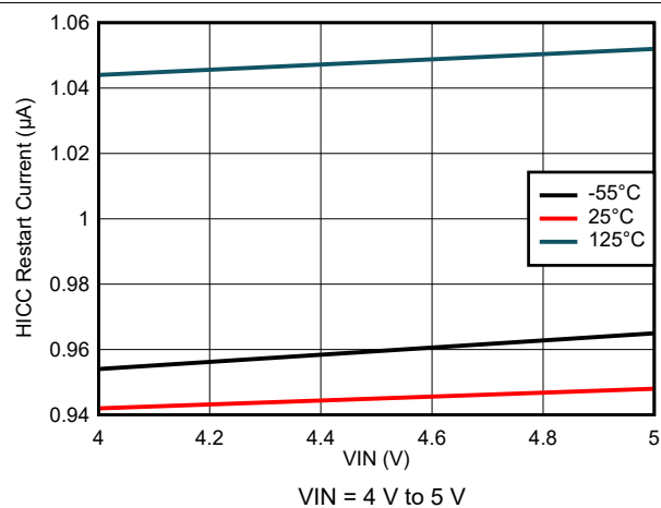
图 8-29. Hiccup Restart Current Variation
