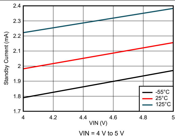
图 8-3. Standby Current Variation
