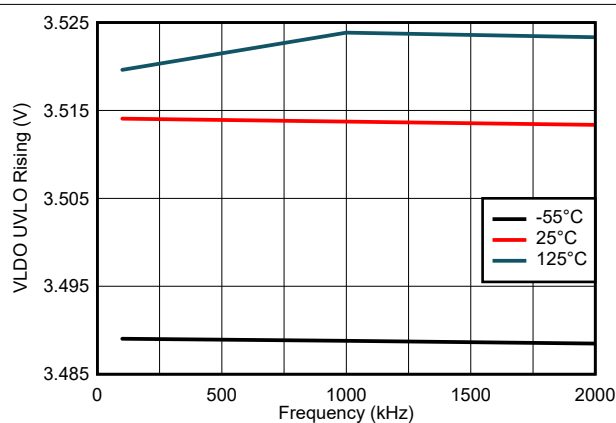
图 8-5. VLDO UVLO Rising Variation
