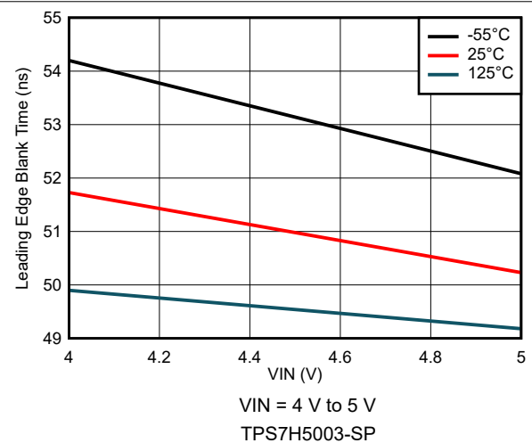
图 8-39. Leading Edge Blank Time Variation
