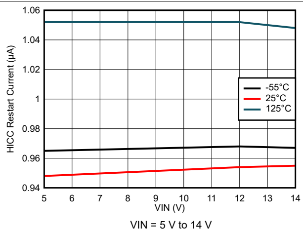
图 8-30. Hiccup Restart Current Variation
