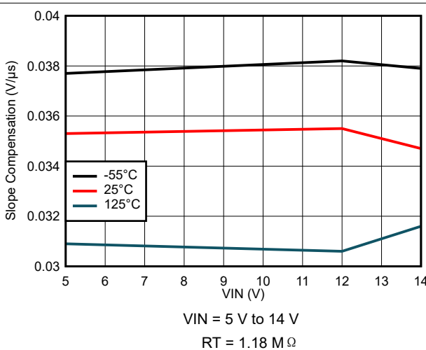
图 8-66. Slope Compensation Variation
