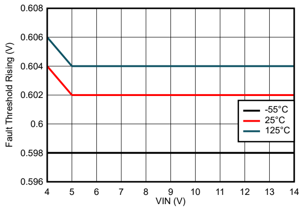
图 8-31. FAULT Threshold Rising Variation
