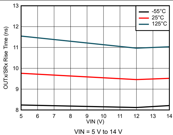
图 8-58. Output Rise Time Variation
