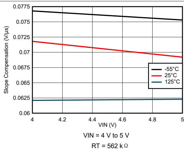
图 8-67. Slope Compensation Variation
