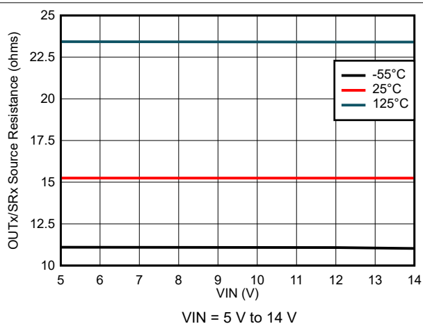
图 8-62. Output Source Resistance Variation
