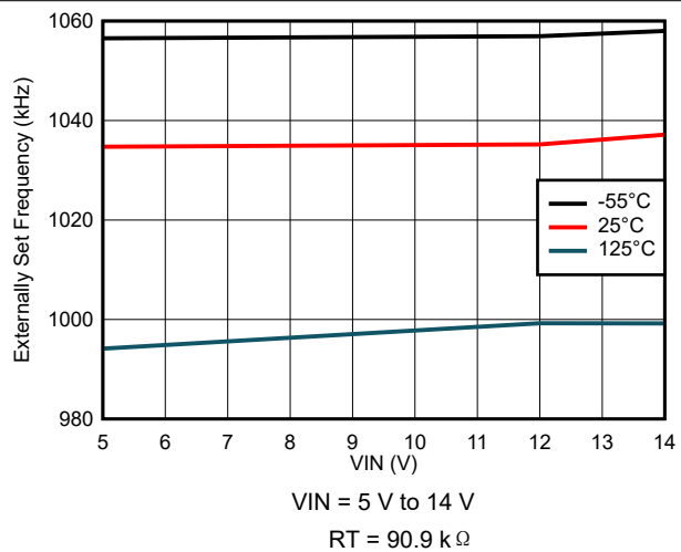
图 8-24. Externally Set Frequency Variation
