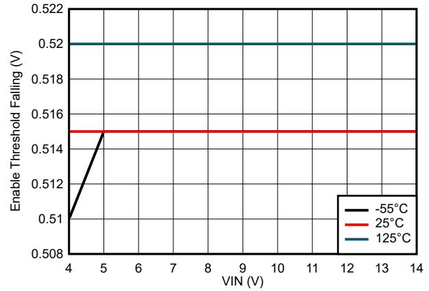
图 8-8. Enable Threshold Falling Variation
