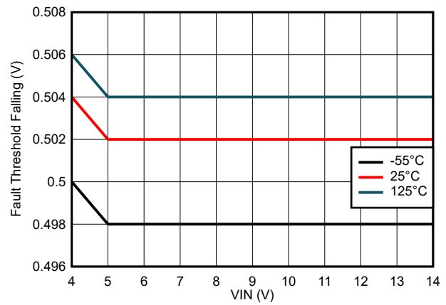
图 8-32. FAULT Threshold Falling Variation
