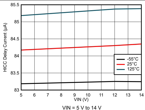
图 8-28. Hiccup Delay Current Variation
