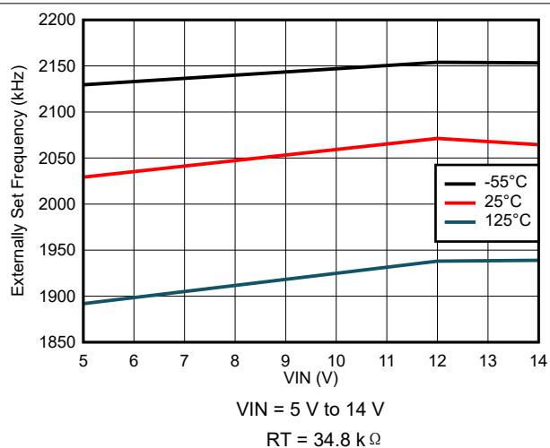
图 8-26. Externally Set Frequency Variation
