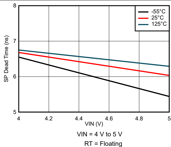
图 8-49. SP Dead Time Variation
