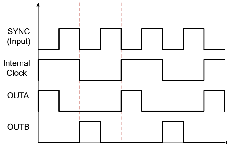
图 9-9. Switching Waveforms for External Synchronization Mode
