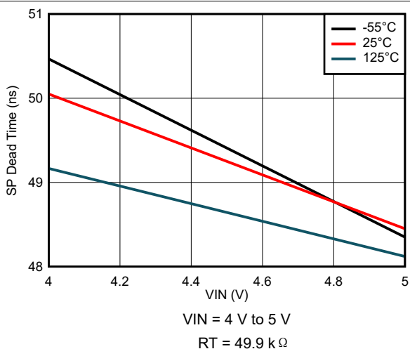
图 8-51. SP Dead Time Variation
