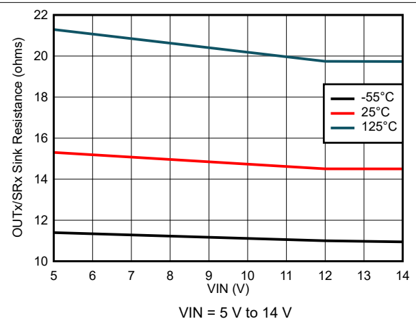
图 8-64. Output Sink Resistance Variation
