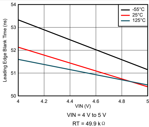
图 8-35. Leading Edge Blank Time Variation
