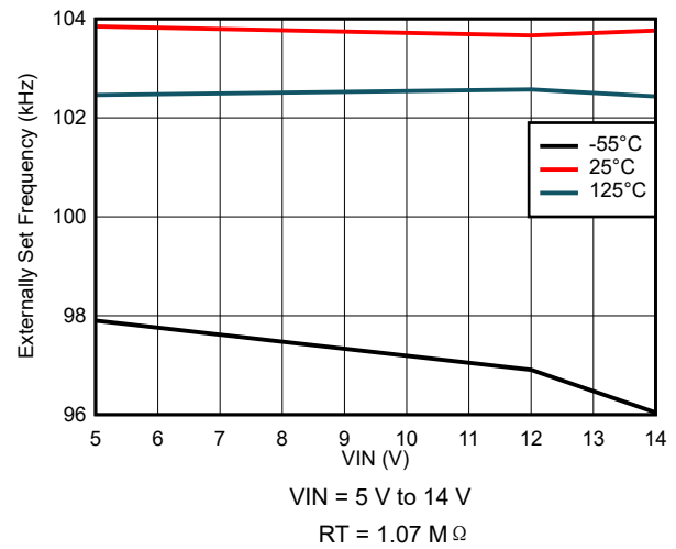
图 8-20. Externally Set Frequency Variation
