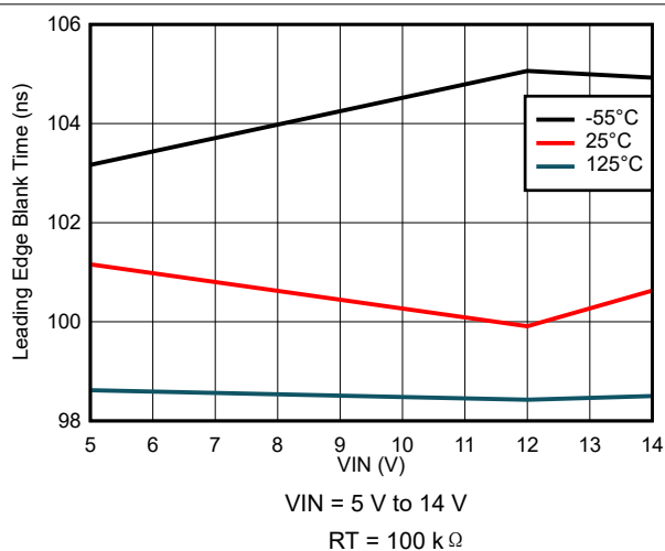
图 8-38. Leading Edge Blank Time Variation
