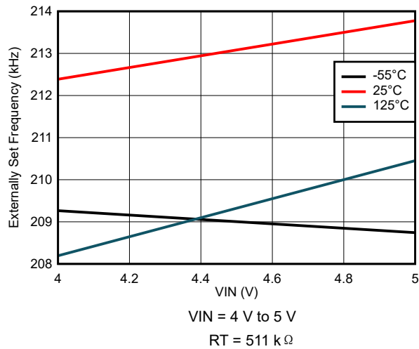
图 8-21. Externally Set Frequency Variation
