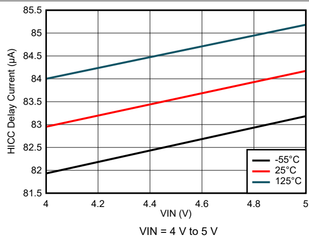
图 8-27. Hiccup Delay Current Variation
