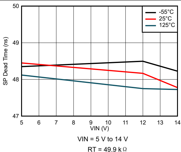
图 8-52. SP Dead Time Variation
