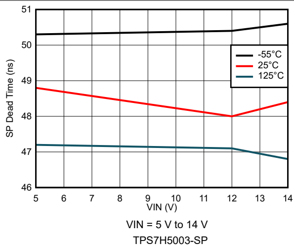
图 8-56. SP Dead Time Variation
