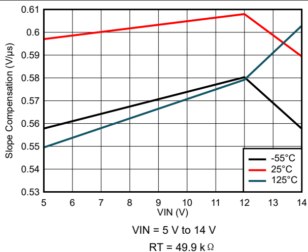
图 8-72. Slope Compensation Variation
