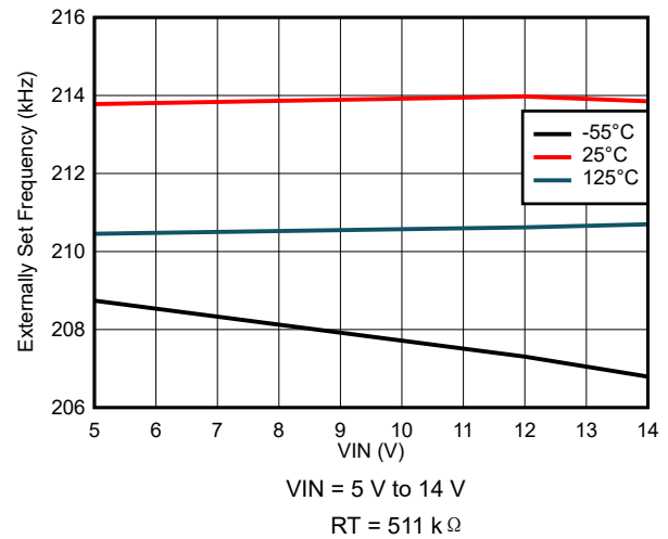
图 8-22. Externally Set Frequency Variation
