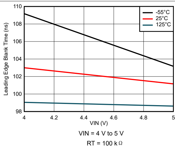
图 8-37. Leading Edge Blank Time Variation
