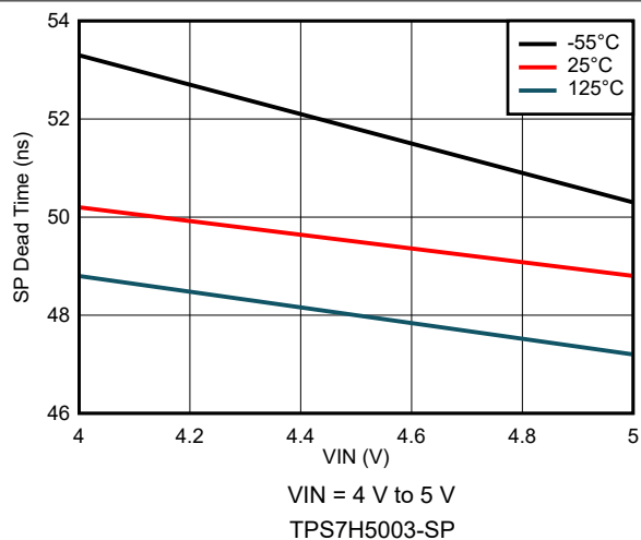
图 8-55. SP Dead Time Variation
