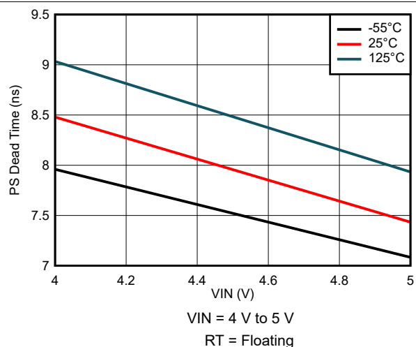
图 8-41. PS Dead Time Variation
