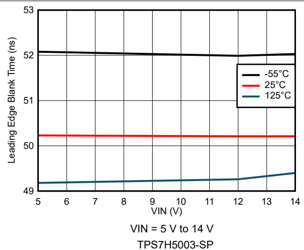
图 8-40. Leading Edge Blank Time Variation
