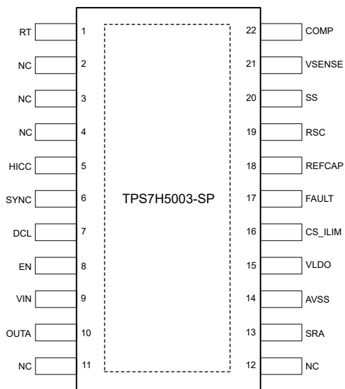
图 7-3. TPS7H5003-SP HFT Package 22-Pin CFP With Thermal Pad (Top View)
