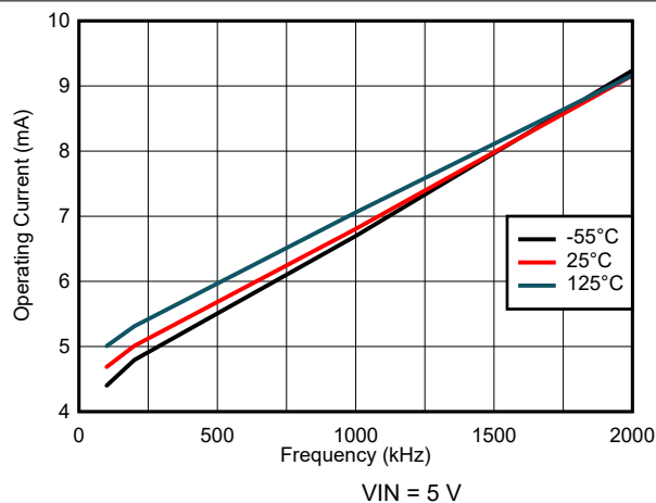
图 8-1. Operating Current Variation
