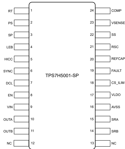
图 7-5. TPS7H5001-SP PW Package 24-Pin TSSOP (Top View)
