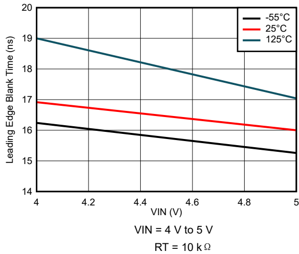
图 8-33. Leading Edge Blank Time Variation
