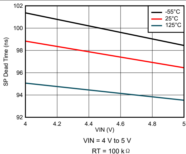
图 8-53. SP Dead Time Variation
