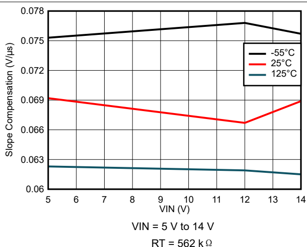
图 8-68. Slope Compensation Variation
