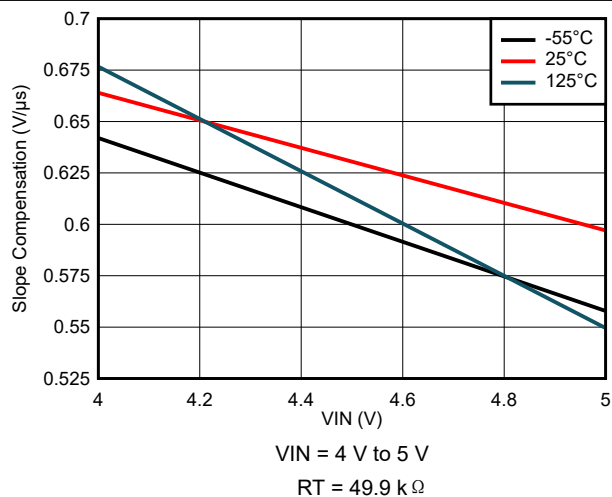
图 8-71. Slope Compensation Variation
