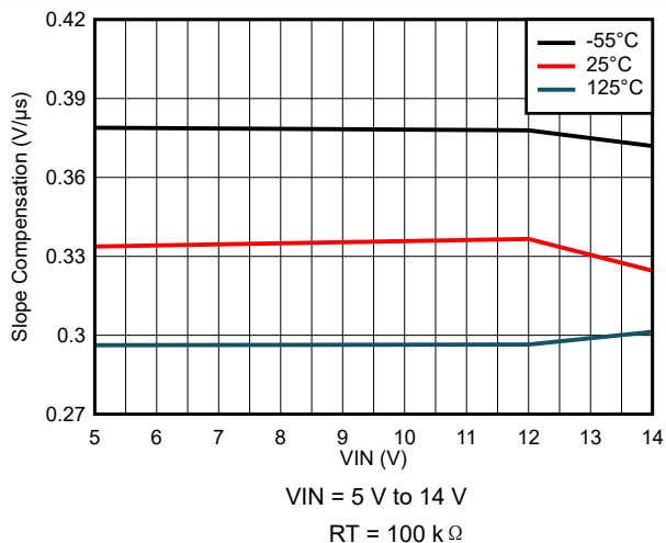
图 8-70. Slope Compensation Variation
