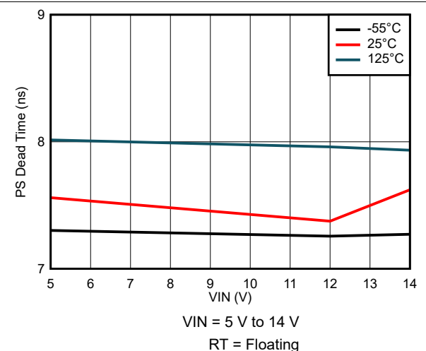
图 8-42. PS Dead Time Variation
