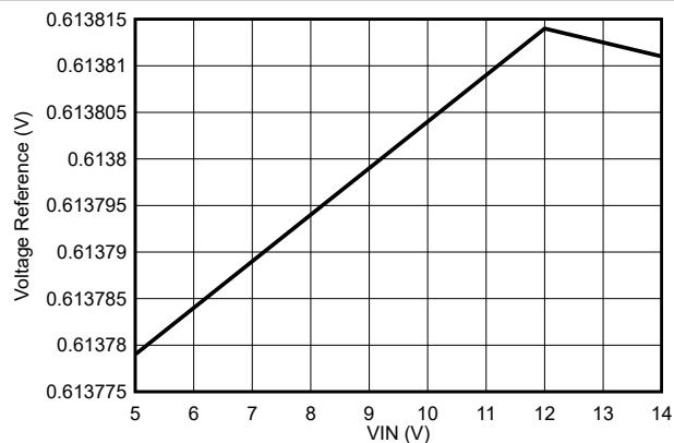
图 8-14. Voltage Reference Variation
