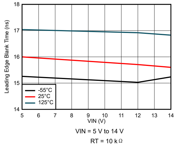
图 8-34. Leading Edge Blank Time Variation
