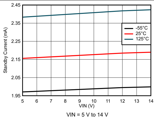
图 8-4. Standby Current Variation
