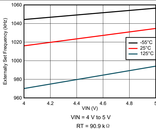
图 8-23. Externally Set Frequency Variation
