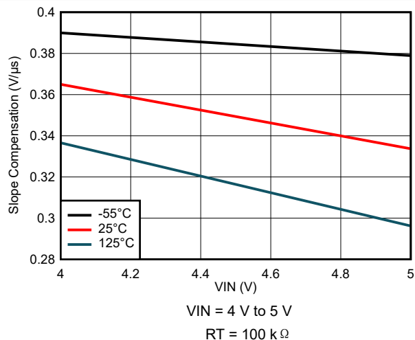
图 8-69. Slope Compensation Variation
