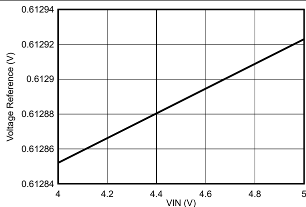
图 8-13. Voltage Reference Variation
