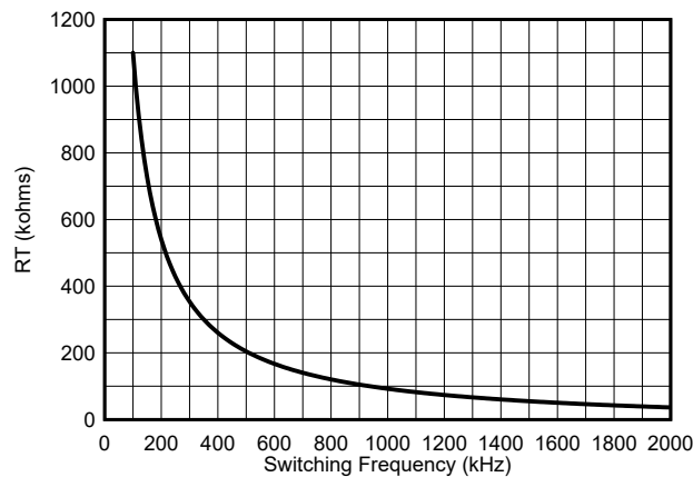
图 9-7. RT vs Switching Frequency
