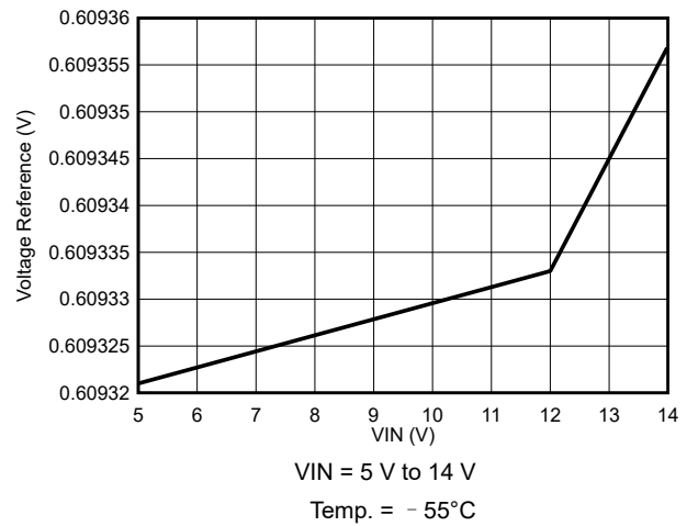
图 8-12. Voltage Reference Variation
