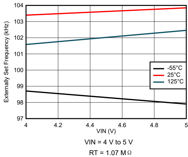
图 8-19. Externally Set Frequency Variation
