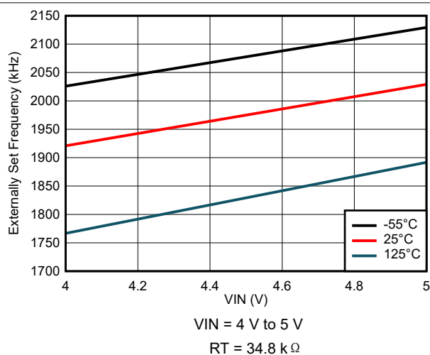
图 8-25. Externally Set Frequency Variation
