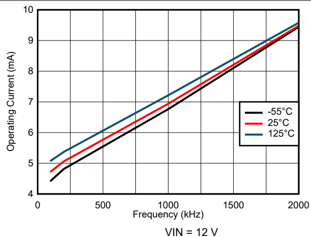
图 8-2. Operating Current Variation
