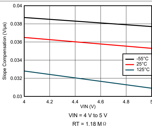
图 8-65. Slope Compensation Variation
