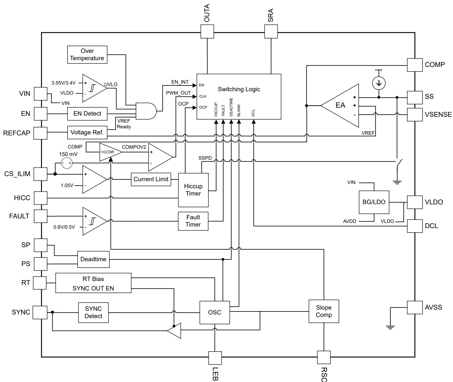
图 9-2. TPS7H5002-SP Functional Block Diagram
