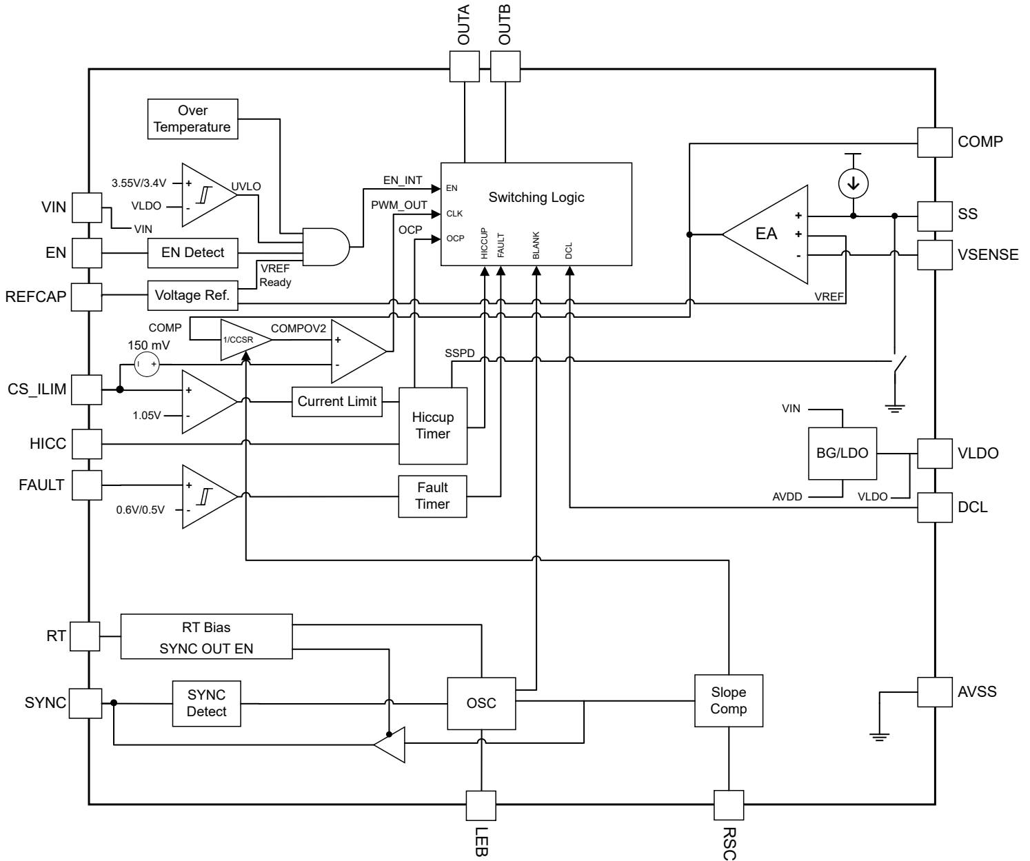
图 9-4. TPS7H5004-SP Functional Block Diagram
