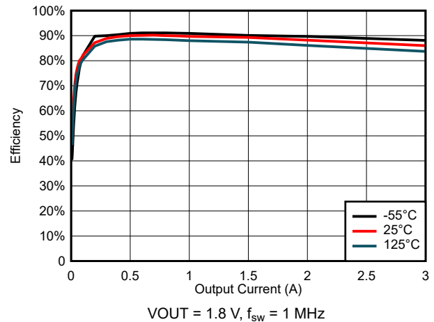
图 6-26. Efficiency for V_{\text{IN}} = 3 \text{ V}
