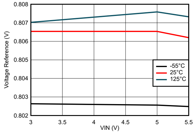
图 6-1. Voltage Reference Variation
