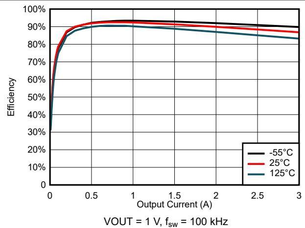
图 6-46. Efficiency for V_{\text{IN}} = 5.5 \text{ V}
