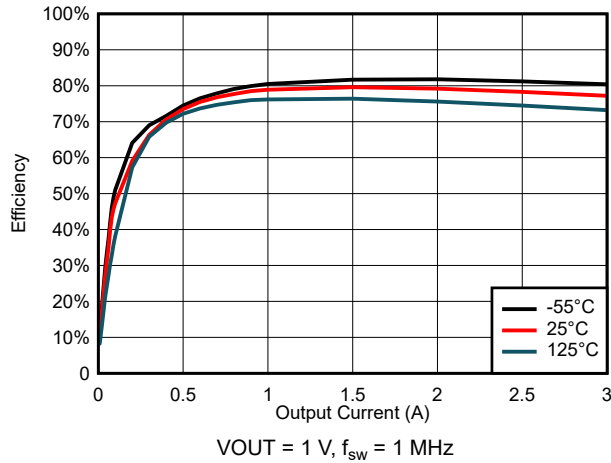
图 6-41. Efficiency for V_{\text{IN}} = 5 \text{ V}
