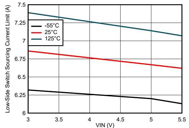
图 6-12. Low-Side Switch Sourcing Current Limit Variation
