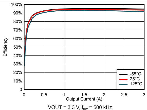
图 6-40. Efficiency for VIN = 5 V
