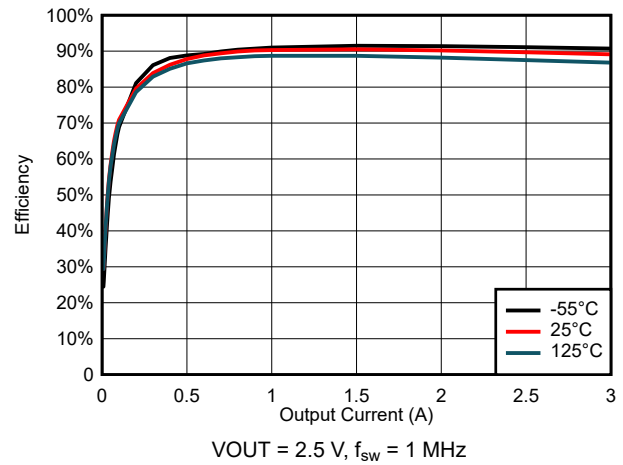
图 6-44. Efficiency for V_{\text{IN}} = 5 \text{ V}
