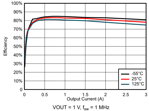
图 6-24. Efficiency for V_{\text{IN}} = 3 \text{ V}
