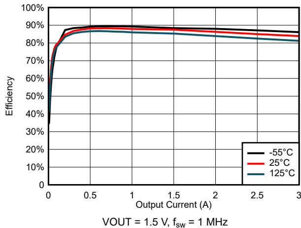
图 6-25. Efficiency for V_{\text{IN}} = 3 \text{ V}
