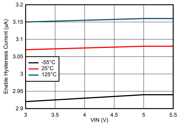
图 6-5. Enable Hysteresis Current Variation
