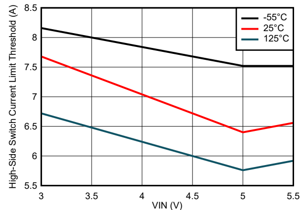
图 6-11. High-Side Switch Current Limit Threshold Variation
