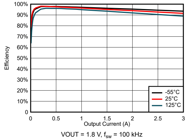
图 6-18. Efficiency for V_{\text{IN}} = 3 \text{ V}
