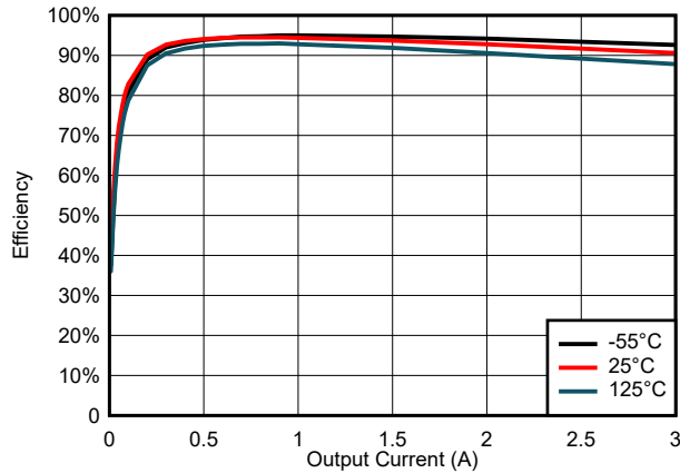
图 6-47. Efficiency for V_{\text{IN}} = 5.5 \text{ V}
