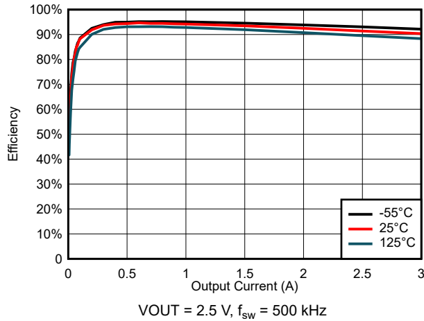
图 6-23. Efficiency for V_{\text{IN}} = 3 \text{ V}
