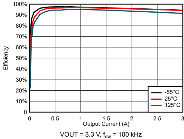
图 6-35. Efficiency for VIN = 5 V
