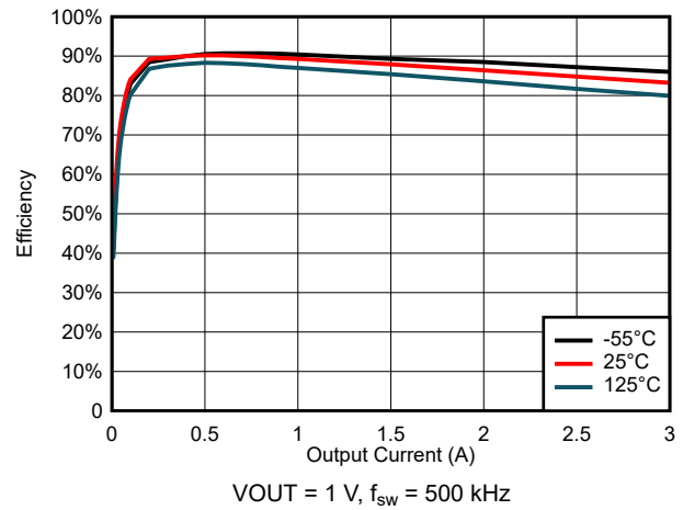
图 6-20. Efficiency for V_{\text{IN}} = 3 \text{ V}
