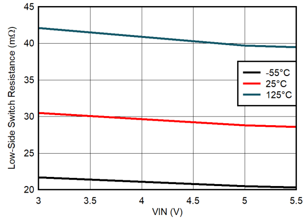
图 6-14. Low-Side Switch Resistance Variation
