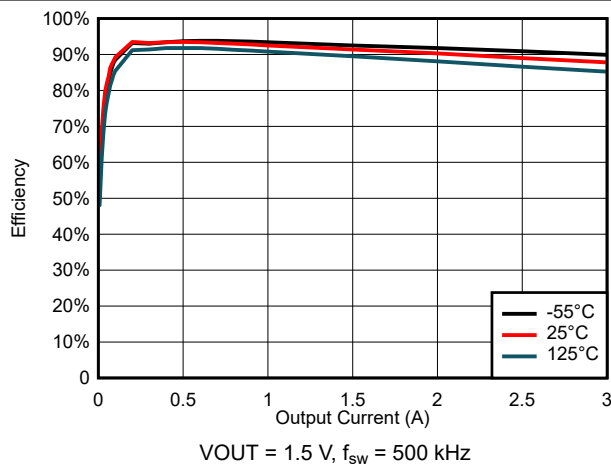
图 6-21. Efficiency for V_{\text{IN}} = 3 \text{ V}
