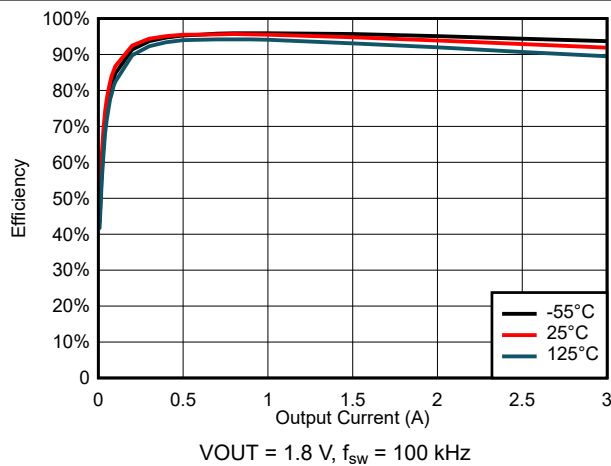
图 6-33. Efficiency for V_{\text{IN}} = 5 \text{ V}
