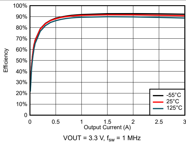
图 6-45. Efficiency for V_{\text{IN}} = 5 \text{ V}
