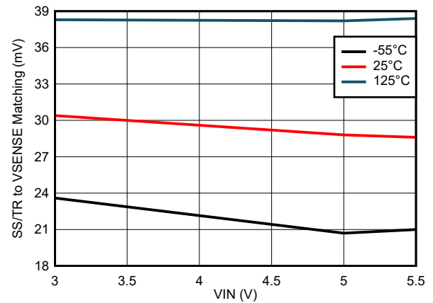
图 6-10. SS/TR to VSENSE Matching Variation
