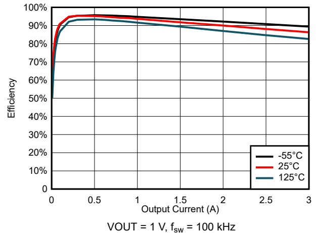
图 6-16. Efficiency for VIN = 3 V
