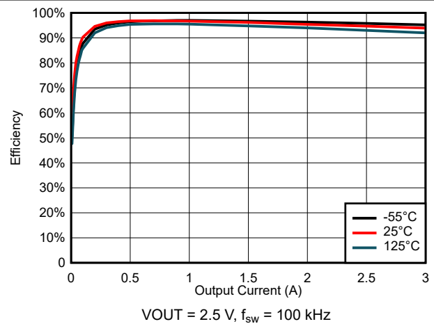
图 6-34. Efficiency for V_{\text{IN}} = 5 \text{ V}
