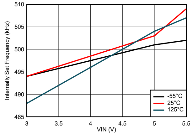
图 6-2. Internally Set Frequency Variation
