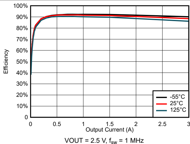
图 6-27. Efficiency for V_{\text{IN}} = 3 \text{ V}
