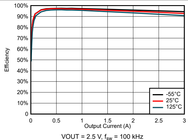
图 6-28. Efficiency for V_{\text{IN}} = 3.3 \text{ V}
