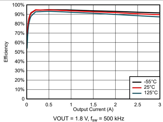
图 6-22. Efficiency for V_{\text{IN}} = 3 \text{ V}
