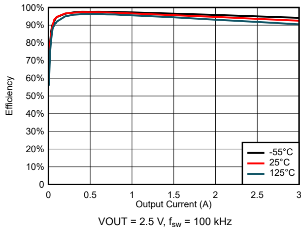
图 6-19. Efficiency for V_{\text{IN}} = 3 \text{ V}
