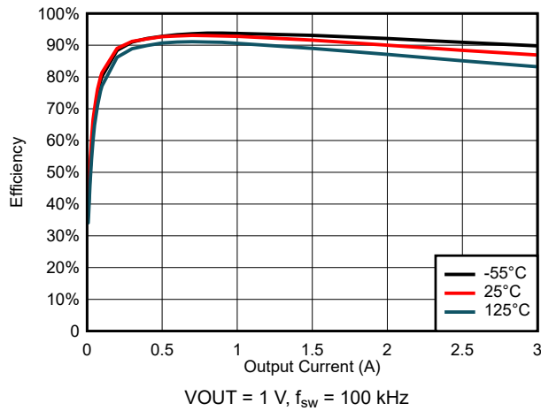
图 6-31. Efficiency for V_{\text{IN}} = 5 \text{ V}
