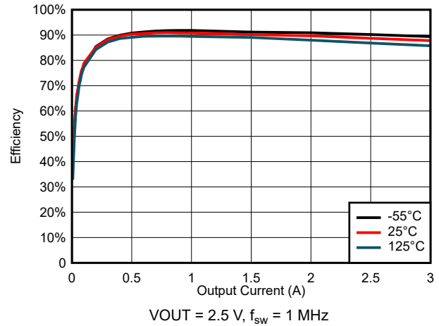
图 6-30. Efficiency for V_{\text{IN}} = 3.3 \text{ V}
