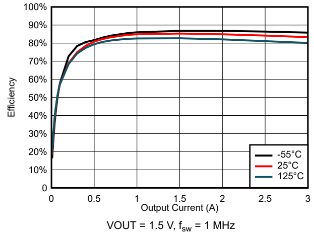
图 6-42. Efficiency for V_{\text{IN}} = 5 \text{ V}
