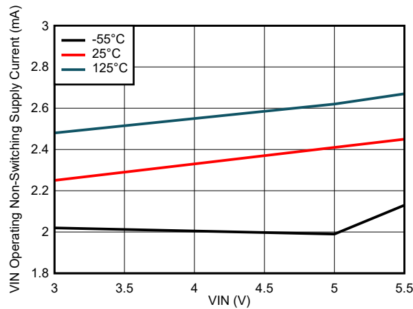
图 6-3. VIN Operating Non-Switching Supply Current Variation
