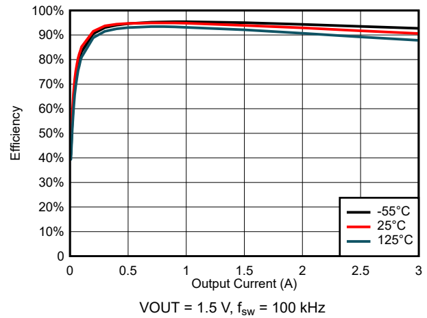
图 6-32. Efficiency for V_{\text{IN}} = 5 \text{ V}
