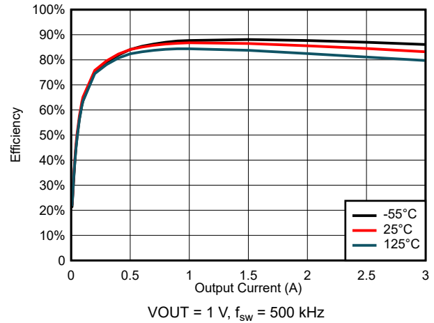
图 6-36. Efficiency for VIN = 5 V
