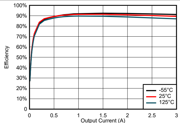
图 6-50. Efficiency for V_{\text{IN}} = 5.5 \text{ V}
