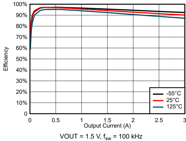
图 6-17. Efficiency for V_{\text{IN}} = 3 \text{ V}
