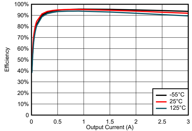
图 6-48. Efficiency for V_{\text{IN}} = 5.5 \text{ V}
