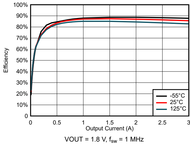
图 6-43. Efficiency for V_{\text{IN}} = 5 \text{ V}
