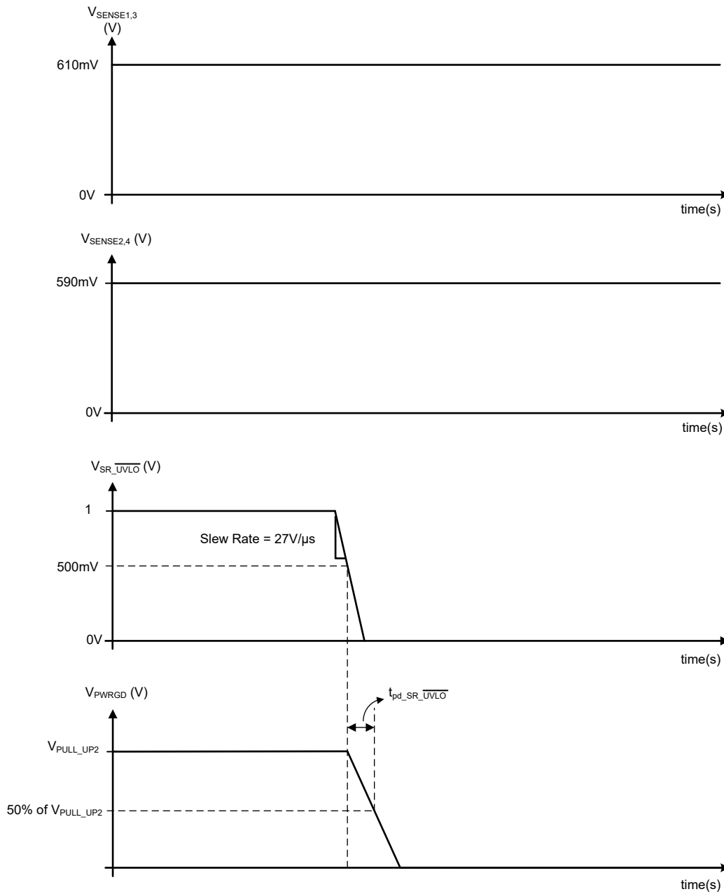
图 7-8. \overline{\text{SR\_UVLO}} 传播延迟 ( t_{\text{pd\_SR\_UVLO}} )
