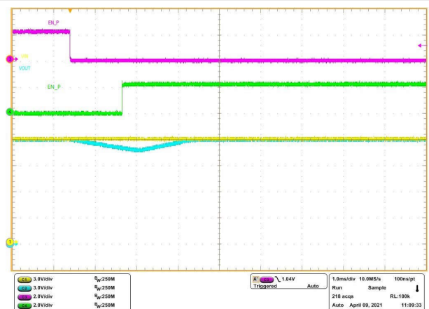
图 10-4. Switch From Primary to Secondary TPS7H2211 in a Cold Sparing Application
