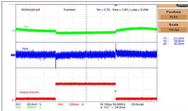
Figure 20. Load Transient Response: Step Load 0 A to 250 \mu A, V_{IN} = 2.3 V, V_{OUT} = 1.8 V
