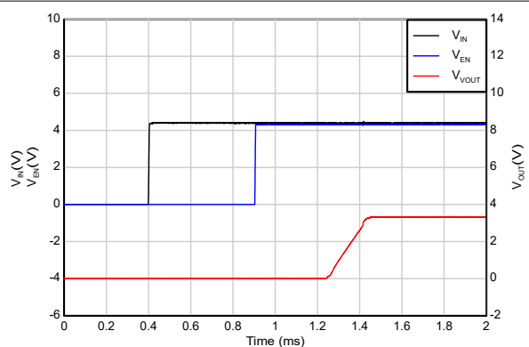
V_{OUT} = 3.3\text{V} , I_{OUT} = 50\text{mA} , 转换率 = 1\text{V}/\mu\text{s}
