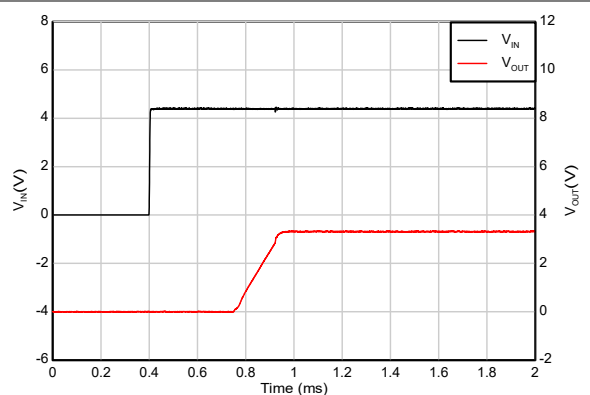
V_{EN} = V_{IN} , V_{OUT} = 3.3\text{V} , 转换率 = 1\text{V}/\mu\text{s}
