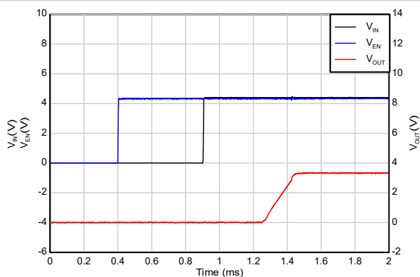
V_{OUT} = 3.3\text{V} , I_{OUT} = 10\text{mA} , 转换率 = 1\text{V}/\mu\text{s}
