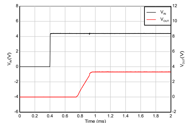
V_{EN} = V_{IN} , V_{OUT} = 3.3\text{V} , I_{OUT} = 10\text{mA} , 转换率 = 1\text{V}/\mu\text{s}
