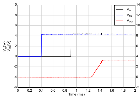
V_{OUT} = 3.3\text{V} , 转换率 = 1\text{V}/\mu\text{s}
