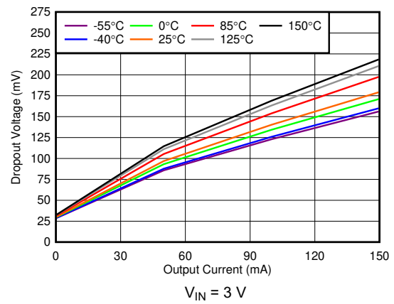
图 5-8. Dropout Voltage ( V_{DO} ) vs I_{OUT}
