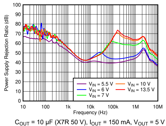
图 5-10. PSRR vs Frequency and V_{IN}
