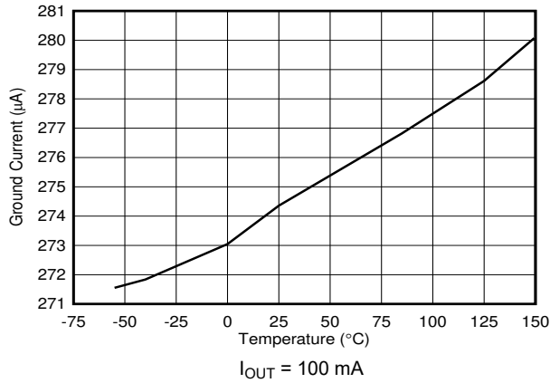
图 5-25. Ground Current
