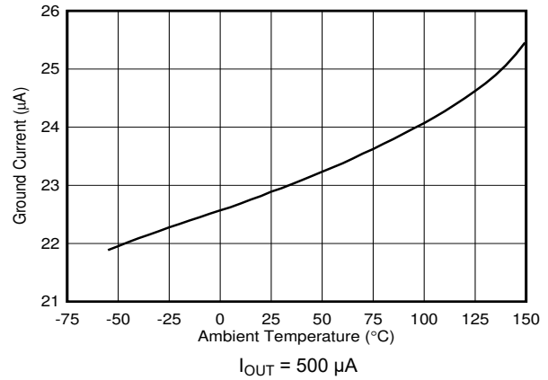
图 5-26. Ground Current
