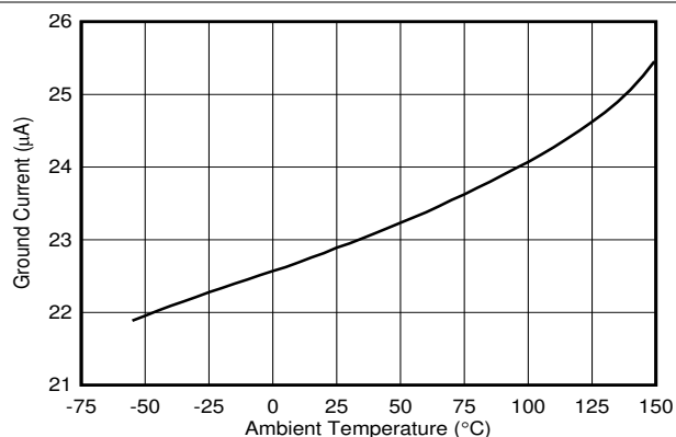
图 6-26. Ground Current
