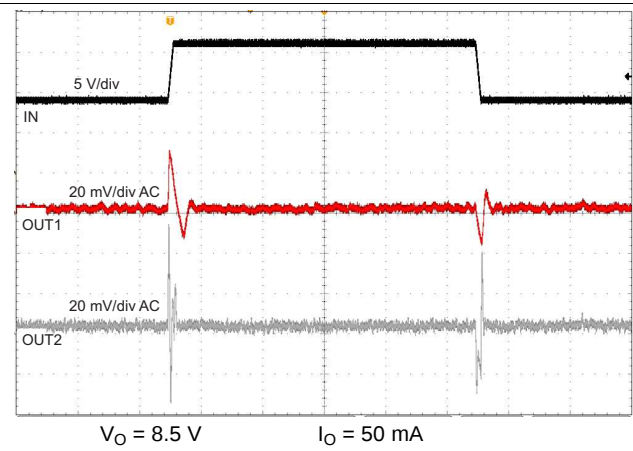
图 14. 9-V to 16-V Line Transient (1 V/μs)
