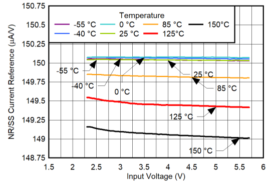
Figure 6-44. I_{NR/SS} vs V_{IN} and Temperature for V_{OUT} = 1.8\text{ V}
