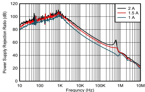
图 8-14. PSRR vs Frequency and I_{OUT} for V_{OUT} = 1.2 V, C_{OUT} = 10 \mu F
