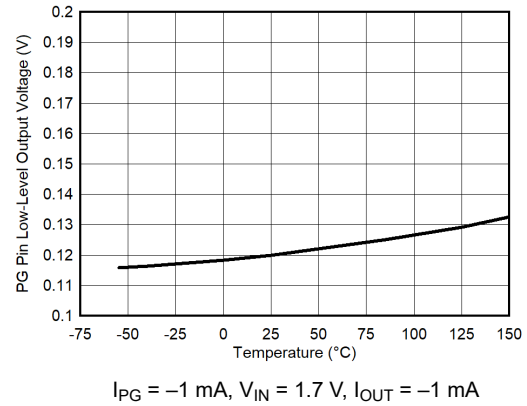
Figure 6-68. V_{PG} Low-Level Output Voltage vs Temperature
