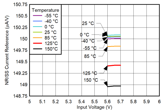
Figure 6-48. I_{NR/SS} vs V_{IN} and Temperature for V_{OUT} = 5.1\text{ V}
