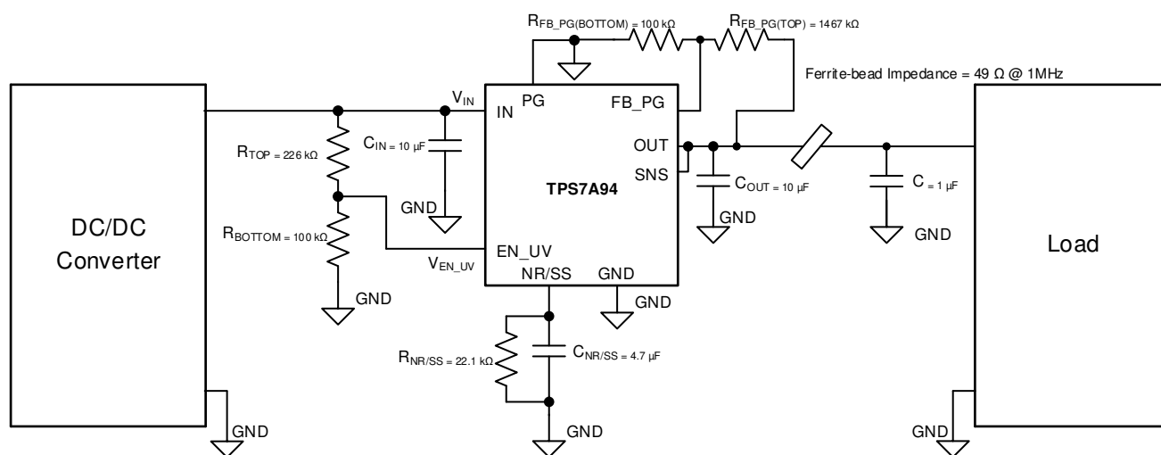
图 8-28. Typical Application Circuit With Added Pi-Filter
