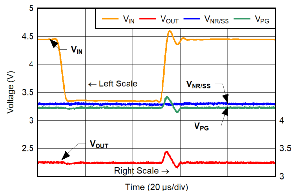
图 8-5. Example: Brownout With Overshoot Recovery
