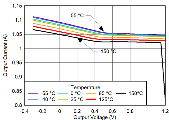
图 6-85. 100% Current Limit vs Temperature for V_{OUT} = 3.3\text{ V}
