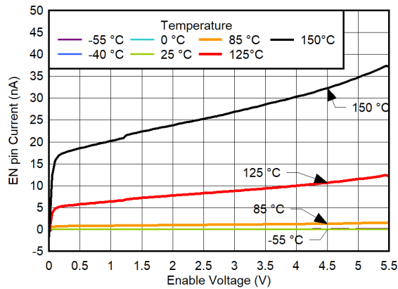
图 6-97. EN Pin Current vs Enable Voltage and Temperature for V_{IN} = 1.7\text{ V}
