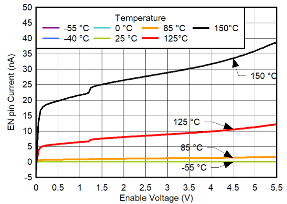
图 6-98. EN Pin Current vs Enable Voltage and Temperature for V_{IN} = 5.7\text{ V}
