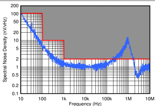
图 8-30. Output Noise vs Frequency
