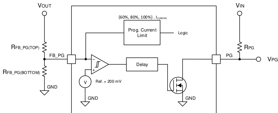
图 8-8. Programmable Power-Good Threshold Simplified Schematic
