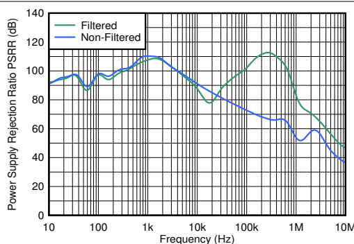
图 8-33. PSRR vs Frequency
