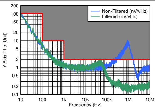
图 8-32. Noise vs Frequency
