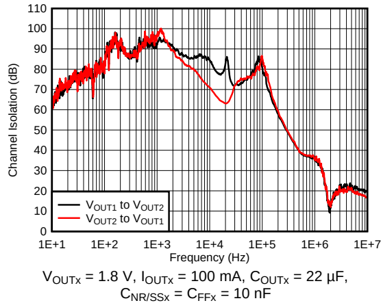
图 7. Channel-to-Channel Output Voltage Isolation vs Frequency
