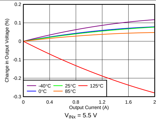
图 28. Load Regulation ( V_{\text{OUTX}} = 5.0\text{ V} )
