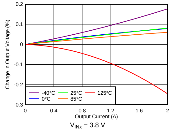
图 26. Load Regulation ( V_{\text{OUTX}} = 3.3\text{ V} )
