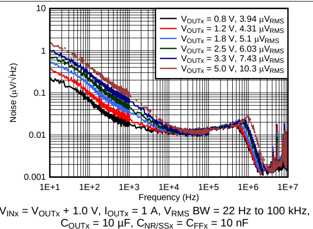
图 10. Noise vs Frequency and Output Voltage
