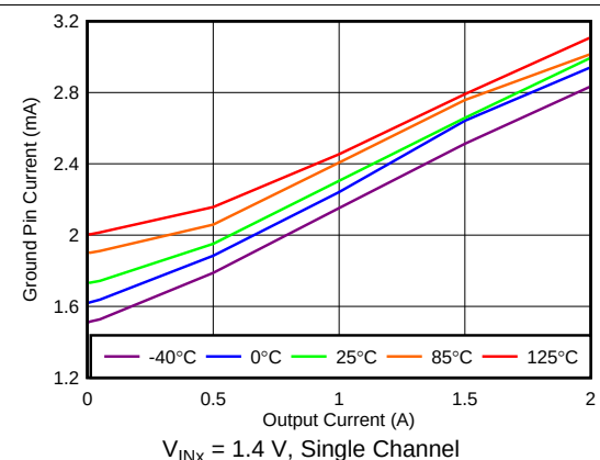
图 30. Ground Current vs Output Current
