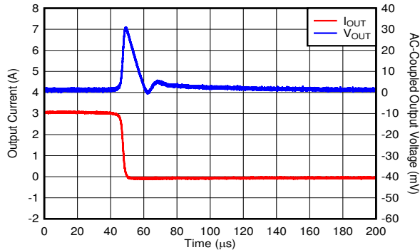
V_{IN} = V_{OUT} + 0.5\text{ V} , V_{OUT} = 0.7\text{ V} , I_{OUT} = 3\text{ A to } 100\text{ mA} , C_{OUT} = 47\ \mu\text{ F} \parallel 10\ \mu\text{ F} \parallel 10\ \mu\text{ F} , C_{NR/SS} = C_{FF} = 10\text{ nF} , slew rate = 1\text{ A}/\mu\text{ s}
