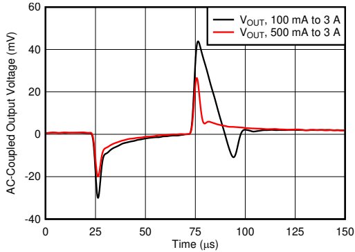
图 6-19. Load Transient vs Time and DC Load
