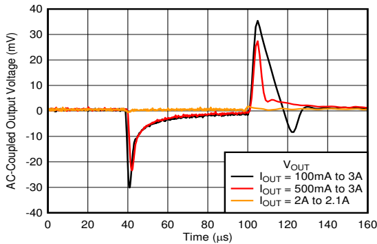
V_{IN} = 1.2\text{ V} , V_{OUT} = 0.7\text{ V} , V_{BIAS} = 5\text{ V} , slew rate = 1\text{ A}/\mu\text{ s} , C_{OUT} = 47\ \mu\text{ F} \parallel 10\ \mu\text{ F} \parallel 10\ \mu\text{ F} , C_{NR/SS} = C_{FF} = 10\text{ nF}
