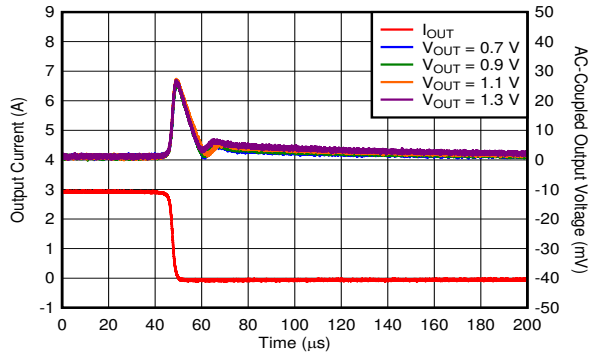
V_{IN} = V_{OUT} + 0.5\text{ V} , V_{BIAS} = 5\text{ V} , I_{OUT} = 3\text{ A to } 100\text{ mA} , slew rate = 1\text{ A}/\mu\text{ s} , C_{NR/SS} = C_{FF} = 10\text{ nF} , C_{OUT} = 47\ \mu\text{ F} \parallel 10\ \mu\text{ F} \parallel 10\ \mu\text{ F}
