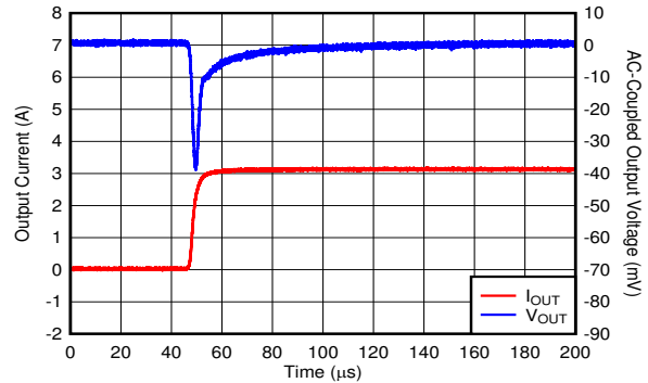
V_{IN} = V_{OUT} + 0.5\text{ V} , V_{OUT} = 0.7\text{ V} , I_{OUT} = 100\text{ mA to } 3\text{ A} , C_{OUT} = 47\ \mu\text{ F} \parallel 10\ \mu\text{ F} \parallel 10\ \mu\text{ F} , C_{NR/SS} = C_{FF} = 10\text{ nF} , slew rate = 1\text{ A}/\mu\text{ s}
