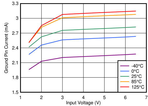
图 6-32. Ground Pin Current vs V_{IN} V_{BIAS} = 0\text{ V} , I_{OUT} = 5\text{ mA}
