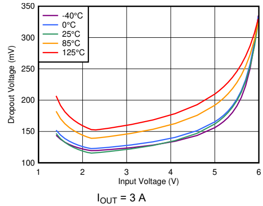
图 6-20. Dropout Voltage vs V_{IN} Without Bias
