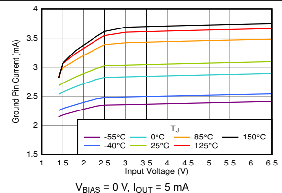
图 6-78. Ground Pin Current vs V_{IN}
