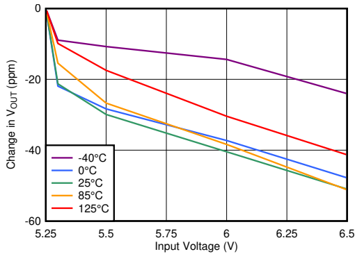
图 6-31. Line Regulation vs V_{IN} (5-V Output) I_{OUT} = 5\text{ mA}
