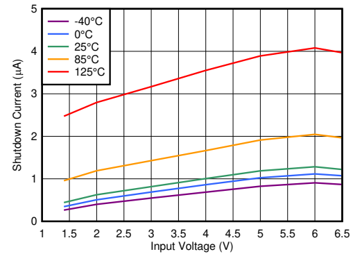
图 6-34. Shutdown Current vs V_{IN} V_{BIAS} = 0\text{ V}
