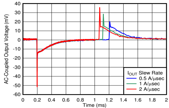
V_{OUT} = 5\text{ V} , I_{OUT,DC} = 100\text{ mA} , I_{OUT} = 100\text{ mA to } 3\text{ A} , C_{OUT} = 47\ \mu\text{ F} \parallel 10\ \mu\text{ F} \parallel 10\ \mu\text{ F} , C_{NR/SS} = C_{FF} = 10\text{ nF}
