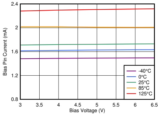
图 6-33. Bias Pin Current vs Bias Voltage V_{IN} = 1.1\text{ V} , I_{OUT} = 5\text{ mA}
