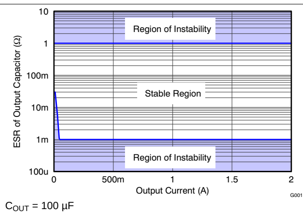
Figure 2. Stability Curve
